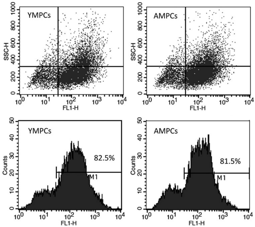
SUPPLEMENTARY FIG. S2. Lentivirus labeling efficiency of MPCs. Flow cytometry was used to determine the GFP-lentivirus labeling efficiency of MPCs isolated from young (YMPCs) and adult (AMPCs) limb muscles. Data are representative for all experiments performed.
