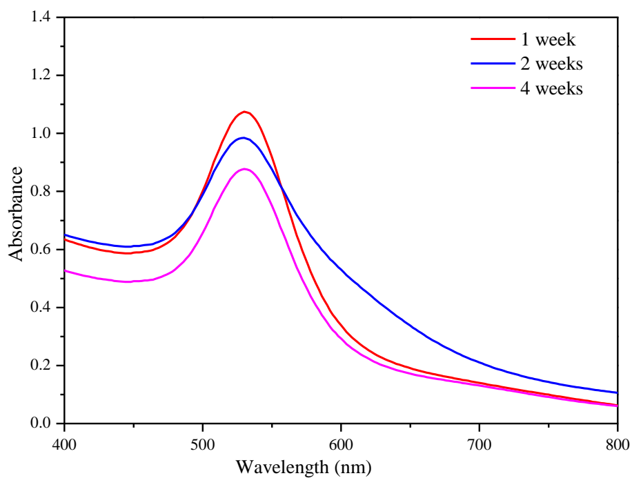
Figure S4. UV-vis spectra of CAO-AuNPs of four weeks stability at different times.
