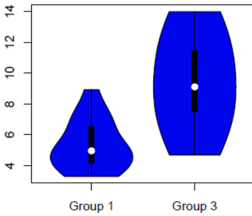
Cmax d-MPH Group 1 vs Group 3
