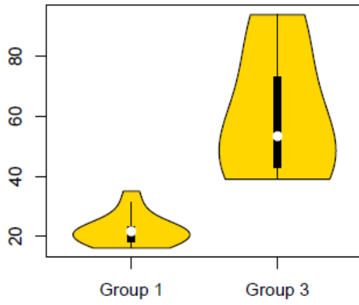
AUC d-MPH Group 1 vs Group 3
