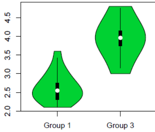
Half life d-MPH Group 1 vs Group 3
