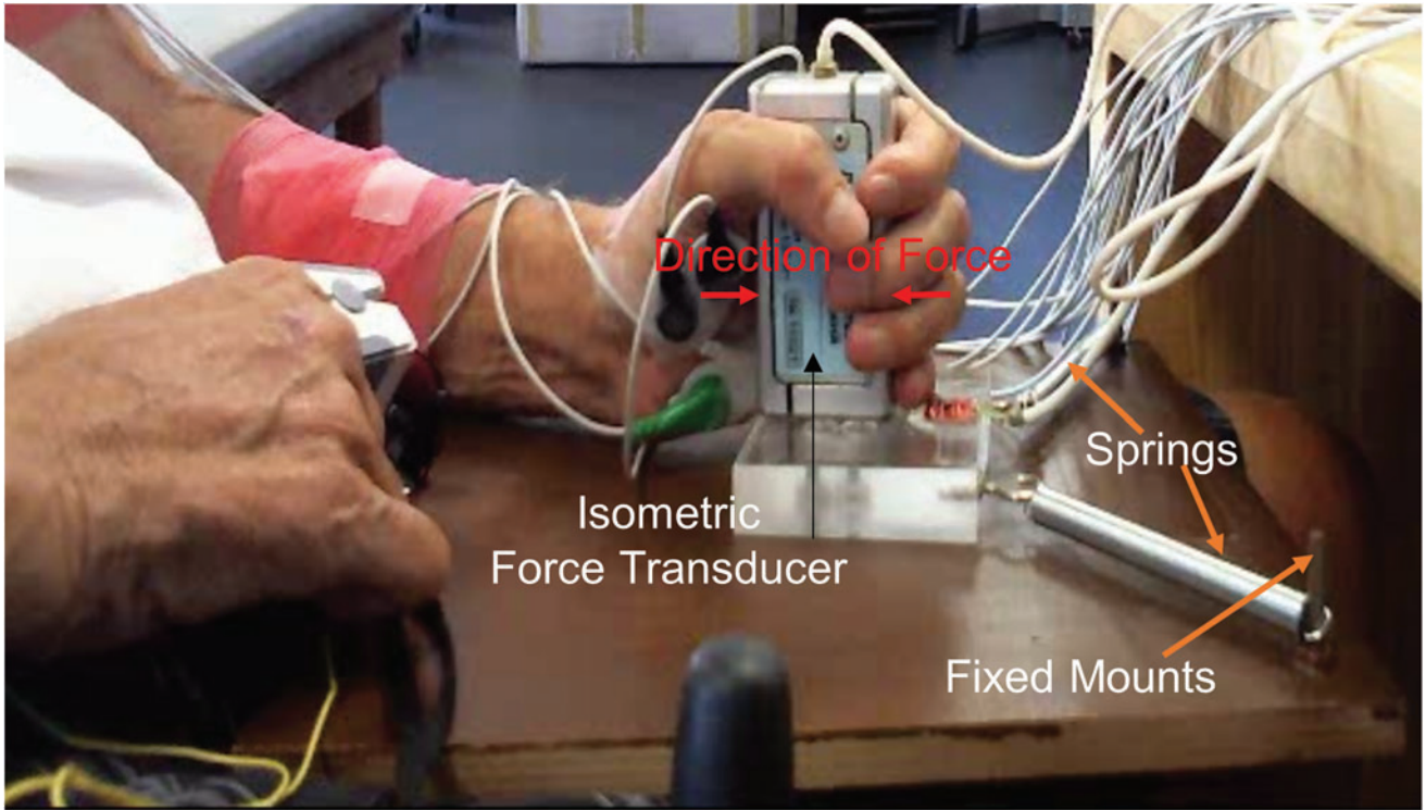
SUPPLEMENTARY FIG. 2. Image of the custom built setup including the isometric force transducer.
