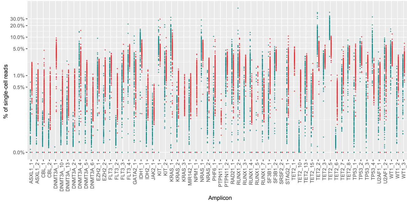
Supplemental Figure S1. Uniformity of amplification across the 62 amplicon AML panel. The percentage of total reads per cell is plotted for each of the 62 amplicons in the targeted AML panel. Each point in the plot represents the data from a single-cell. Blue colored data points were generated for droplet amplification conditions prior to uniformity optimization. Red data points were generated following optimization of thermocycling conditions and reaction components. For each of the two separate conditions the same 250 cells are shown across all of the different sequenced loci.
