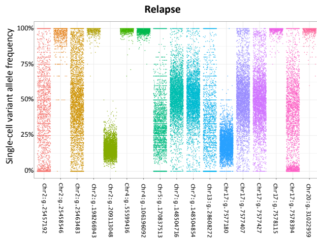
Supplemental Figure S4. Single-cell variant allele frequencies. Single cell VAFs are plotted for all 17 of the identified genetic variants found in the diagnosis, complete remission and relapse samples.
