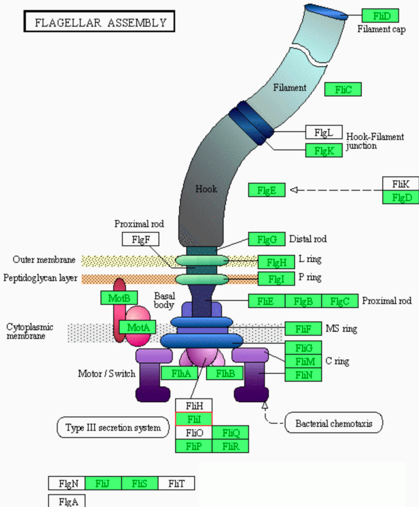
Supplementary Figure 2. Expanded view of the flagellar assembly. Genes encoding relevant proteins that were found in the Ca. Abyssubacteria genomes are highlighted in green. Genes not present are white. Figure generated on the IMG/ER database.
