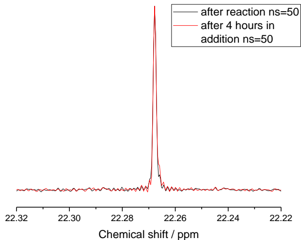
Figure S5.: ^{13}\text{C} NMR spectra with ^1\text{H} decoupling of the hydrogenated flame sealed sample. The peak of the internal standard toluene- \alpha - ^{13}\text{C} is not changed even after several hours. The peak intensities of the internal standard is used to calculate the carbon hyperpolarization enhancement together with the ratio
