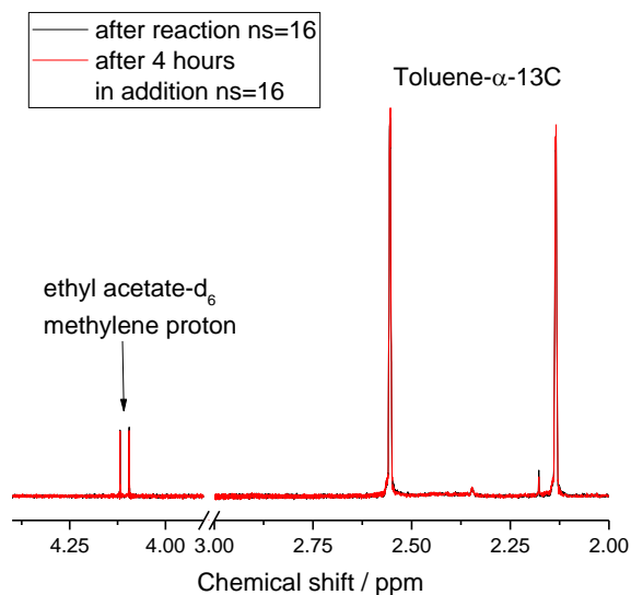
Figure S4.: ^1\text{H} NMR spectra under ^2\text{H} decoupling of the hydrogenated flame sealed sample. The peaks of the internal standard toluene- \alpha - ^{13}\text{C} and the ethyl acetate product are not changed. The peak intensities of the product are used to calculate the proton hyperpolarization, enhancement and ratio between product and internal standard. The relaxation delay between scans was 500 s and 32 scans were acquired.
