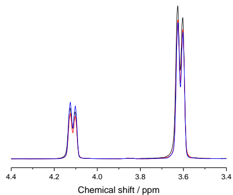
Figure S8.: ^1\text{H} spectra of the 0.45 ml solution 20 s after addition of NaOD. Chemical shifts are calibrated to MeOD (3.34 ppm). Non-cleaved ethyl acetate appears at \sim 4.1 ppm and the cleaved ethanol appears at \sim 3.6 ppm.
