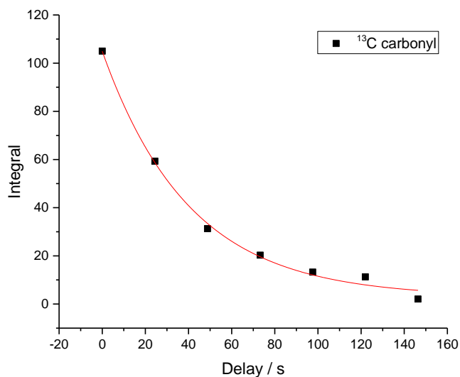
Figure S13 : The relaxation of the ^{13}\text{C} carbonyl magnetization of ethyl acetate- \text{d}_6 was measured at 7 T and 320 K after the para-hydrogen reaction by using small flip angle pulses ( 5.6^\circ ). T_1 = 40 \pm 4\text{s} in methanol- \text{d}_4 .
