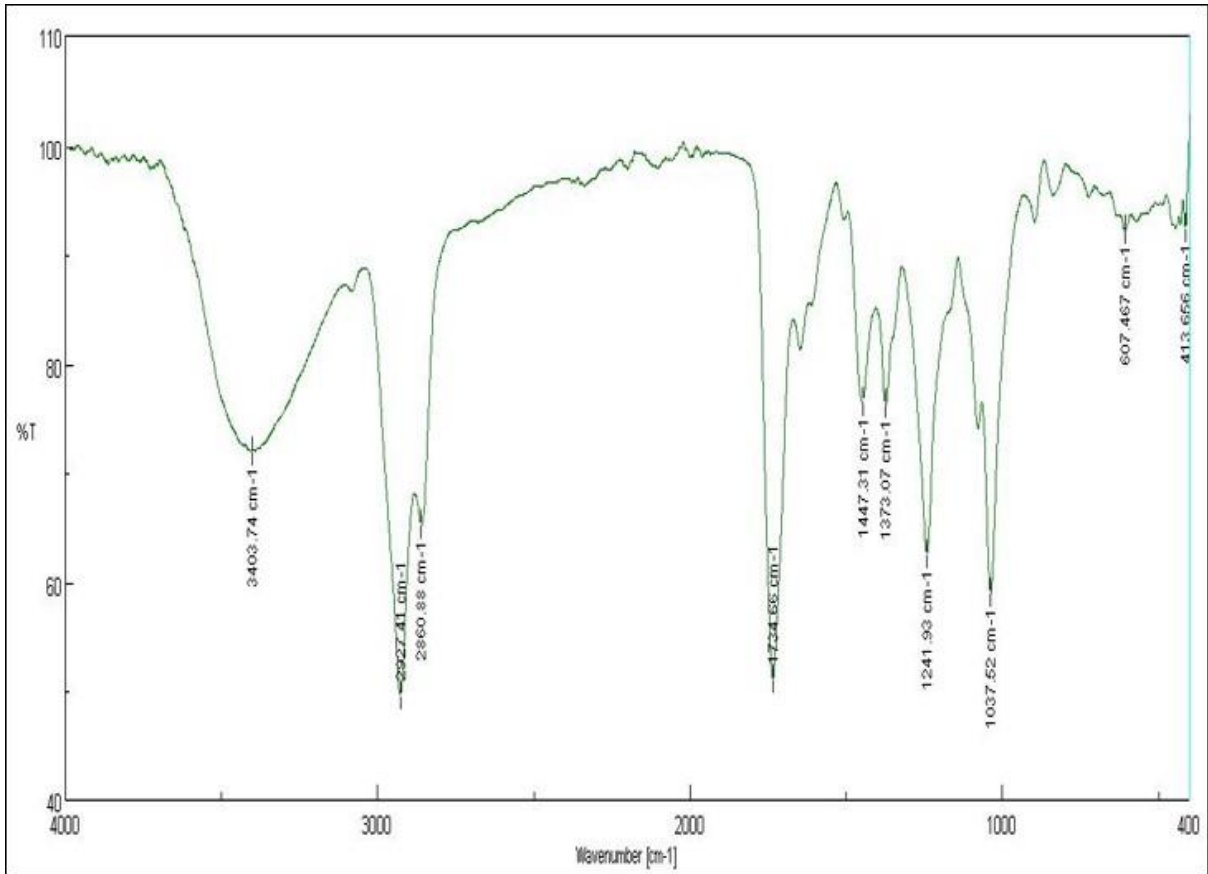
FTIR spectra of CEA extract
