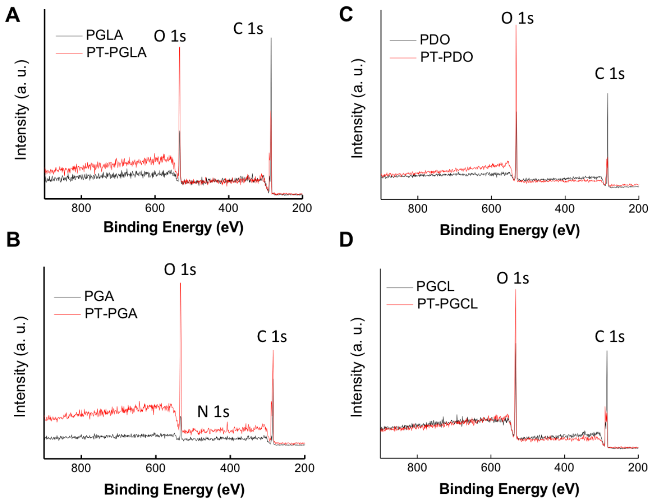
S3 Fig. XPS survey spectra of sutures. XPS survey spectra of (A) PGLA, (B) PGA, (C) PDO and (D) PGCL before and after 7-minute NTAP treatment.
