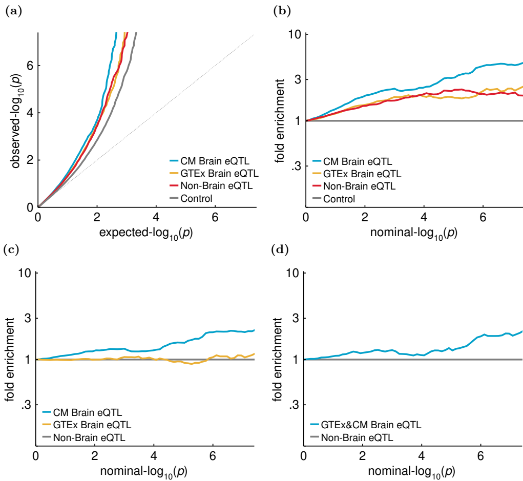
S1 Fig Enrichment plots for CommonMind, GTEX, GTEX/CommonMind consensus brain and non-CNS eQTLs. The top panels contain Q-Q and fold enrichment plots for the CommonMind, GTEX brain and TwinsUK non-CNS eQTLs. The bottom panels contain relative fold enrichment plots for CommonMind and GTEX and for GTEX/CommonMind consensus brain eQTLs compared to non-CNS eQTL variants.
