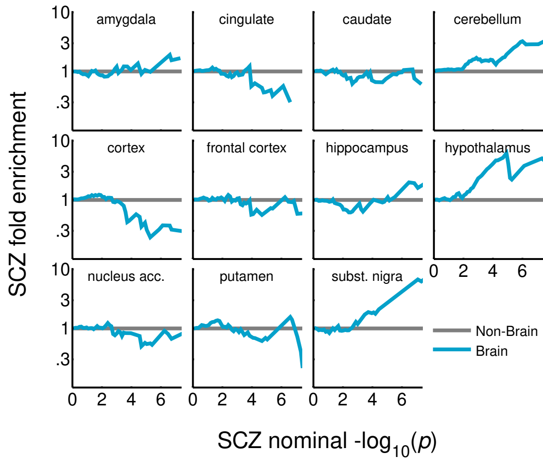
S2 Fig Enrichment plots for GTEx/CommonMind consensus region-specific brain eQTLs. The fold enrichment is relative to non-CNS eQTL variants.
