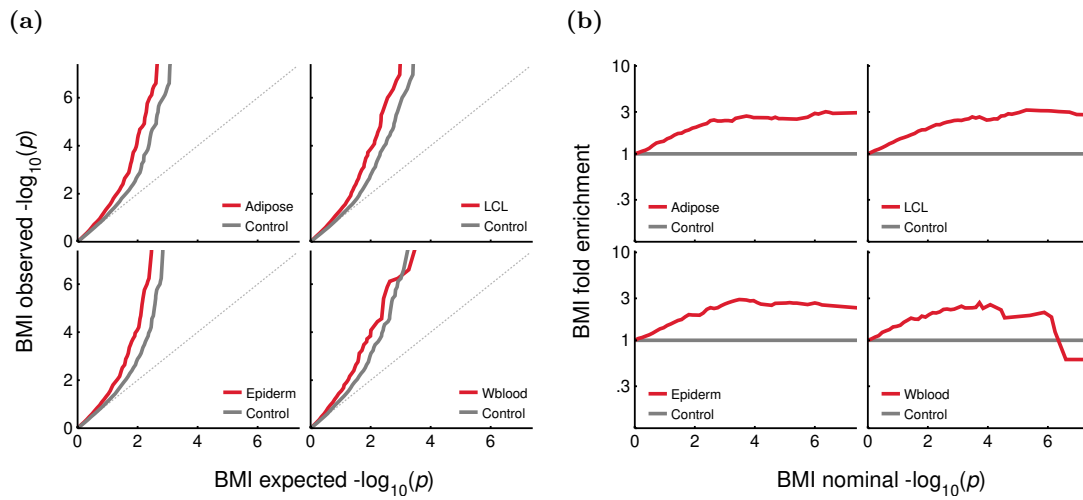
S5 Fig BMI association enrichment in eQTLs. Q-Q and fold enrichment plots for adipose, epidermal, LCL and whole blood eQTLs. The baseline is determined by respectively matched control SNP sets. The fold enrichment is displayed in logarithmic scale.
