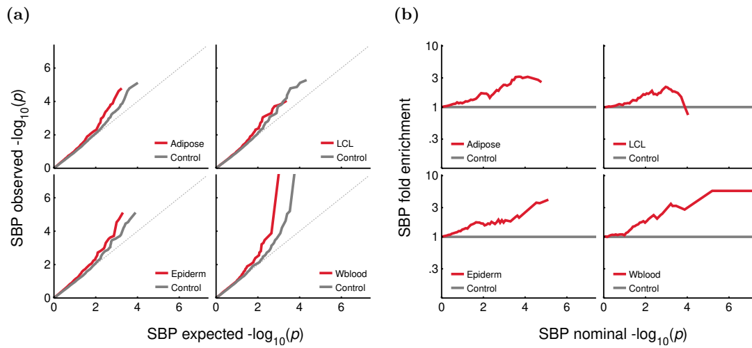
S8 Fig Systolic blood pressure association enrichment in eQTLs. Q-Q and fold enrichment plots for adipose, epidermal, LCL and whole blood eQTLs. The baseline is determined by respectively matched control SNP sets. The fold enrichment is displayed in logarithmic scale.
