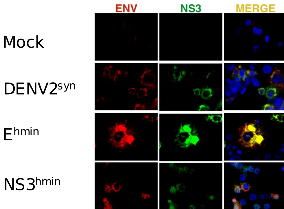
Figure S1. Deconvolution microscopy of THP-1 cells infected with D2-Syn, E hMin , and NS3 hMin or mock infected at an MOI of 5.0. At 2 days post infection, infected cells were fixed and stained using 4G2 anti-E or anti-NS3 primary antibodies as well as FITC (NS3) or Alexa 488 (E) conjugated secondary antibodies.
