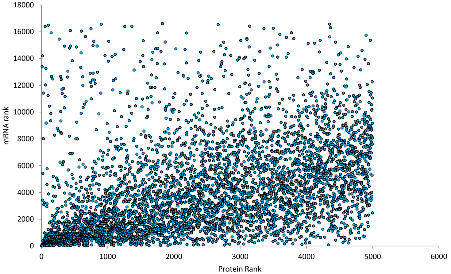
Supplementary Figure 1: Ranked mRNA abundance of genes measured in Sapio et al. plotted versus ranked protein abundance measured in this study.
