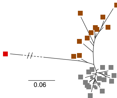
500 SNPs
