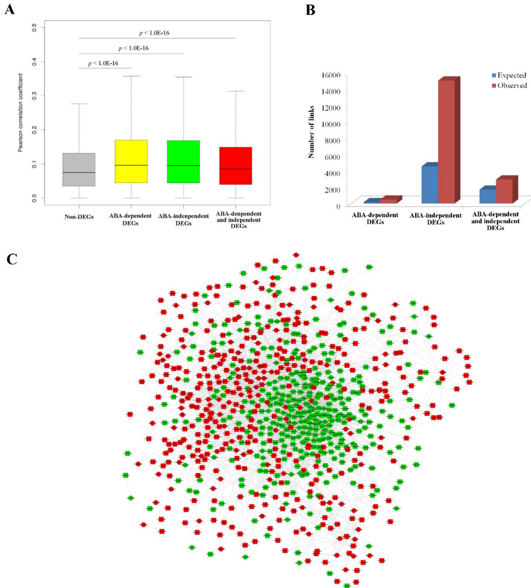
Figure S2 - Co-expression analysis between ABA-dependent and ABA-independent drought-responsive genes.
