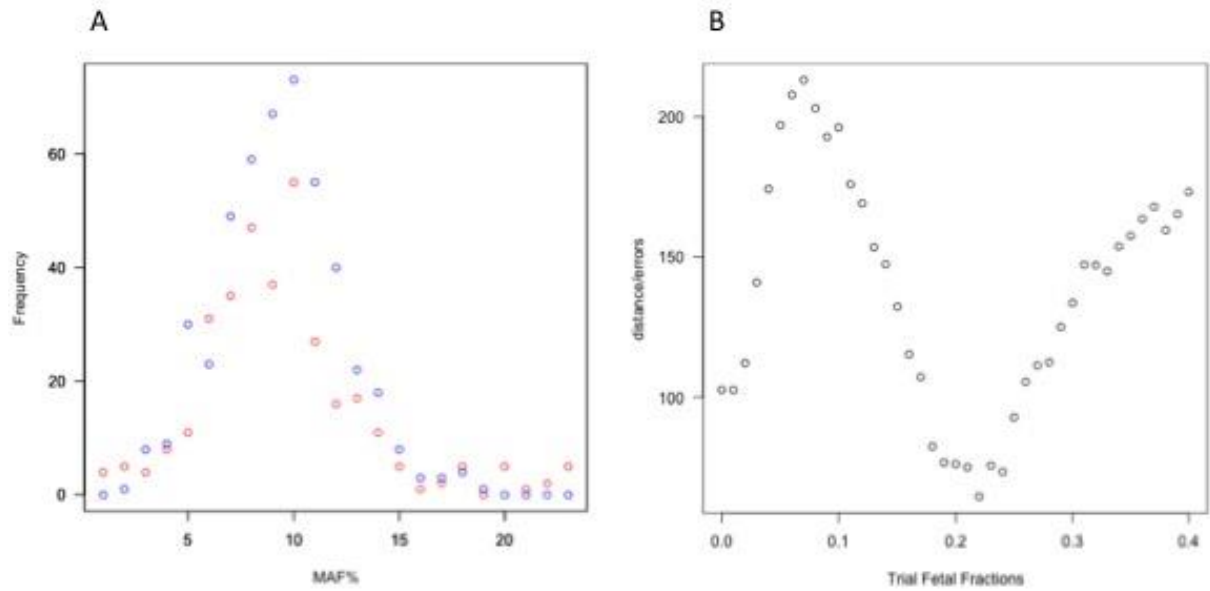
Figure S1 - Fit procedure for FF estimation. A) Distribution of MAF values for both test and simulated samples; Red: test sample; Blue: fitted simulated sample (most similar to the test sample). B) Fitting of the test sample to the closest simulated samples.
