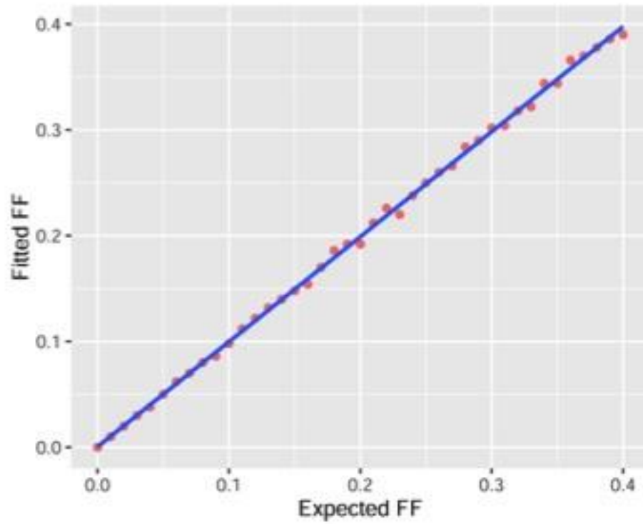
Figure S3 - Evaluation of the fitting for mean coverage value = 150X and SNP numbers = 2000. Shape and color incorporate both mean coverage and SNP number values, respectively
