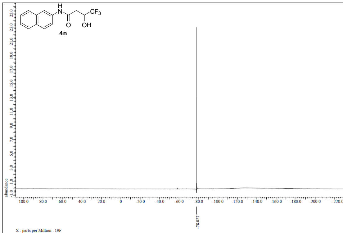
Figure S103. 19 F NMR spectrum of 4n, related to Figure 3.
