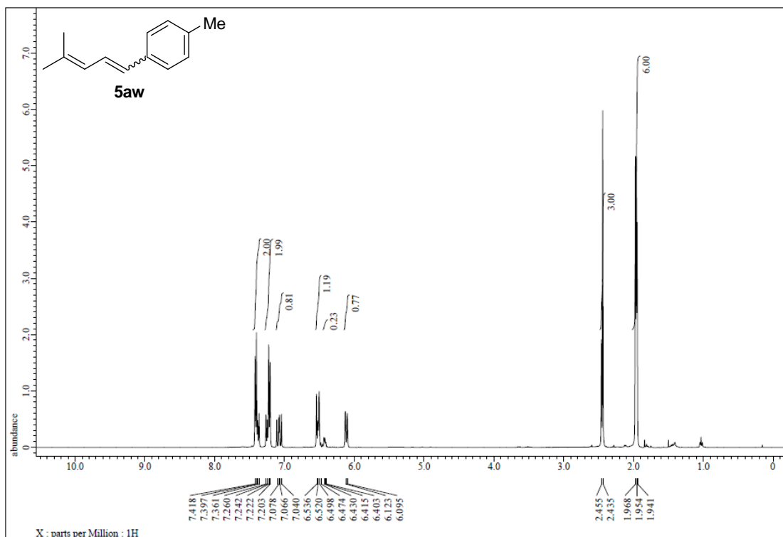
Figure S209. ^1\text{H} NMR spectrum of 5aw, related to Figure 5.
