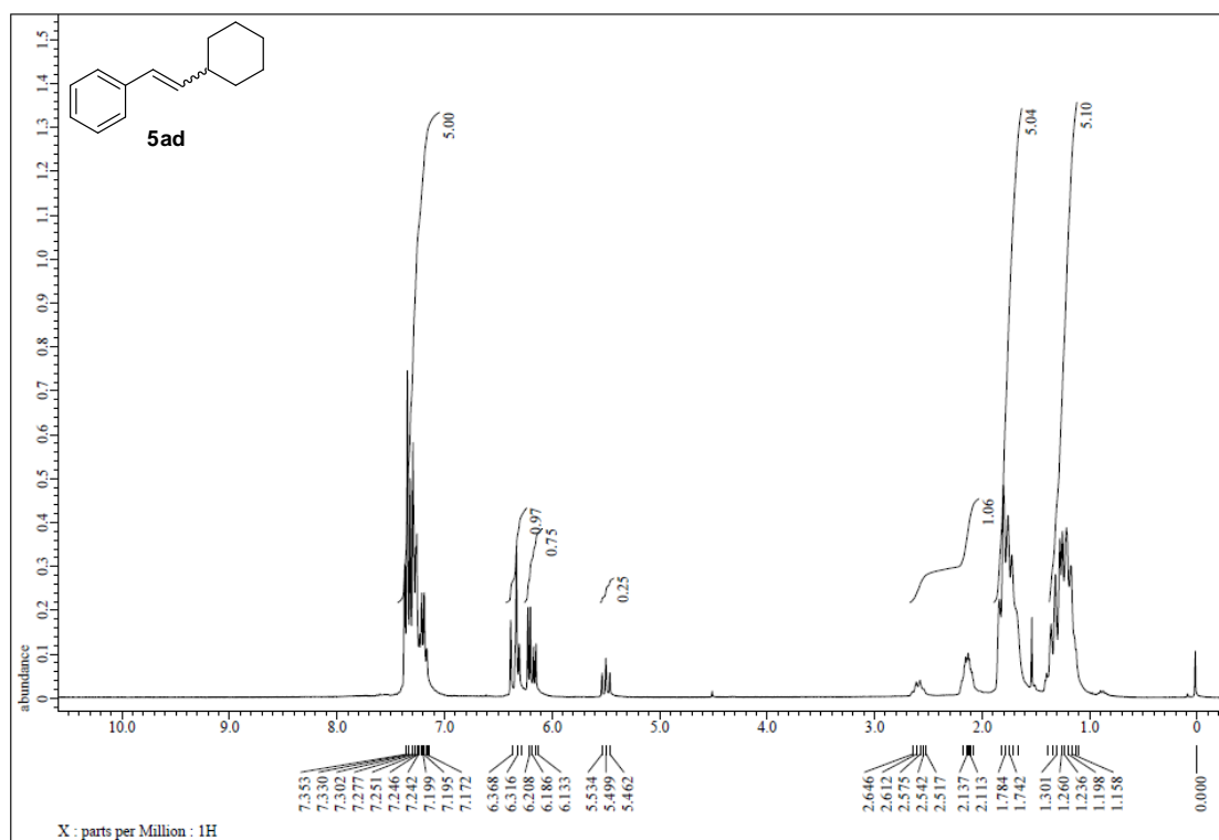
Figure S168. 1 H NMR spectrum of 5ad, related to Figure 4.
