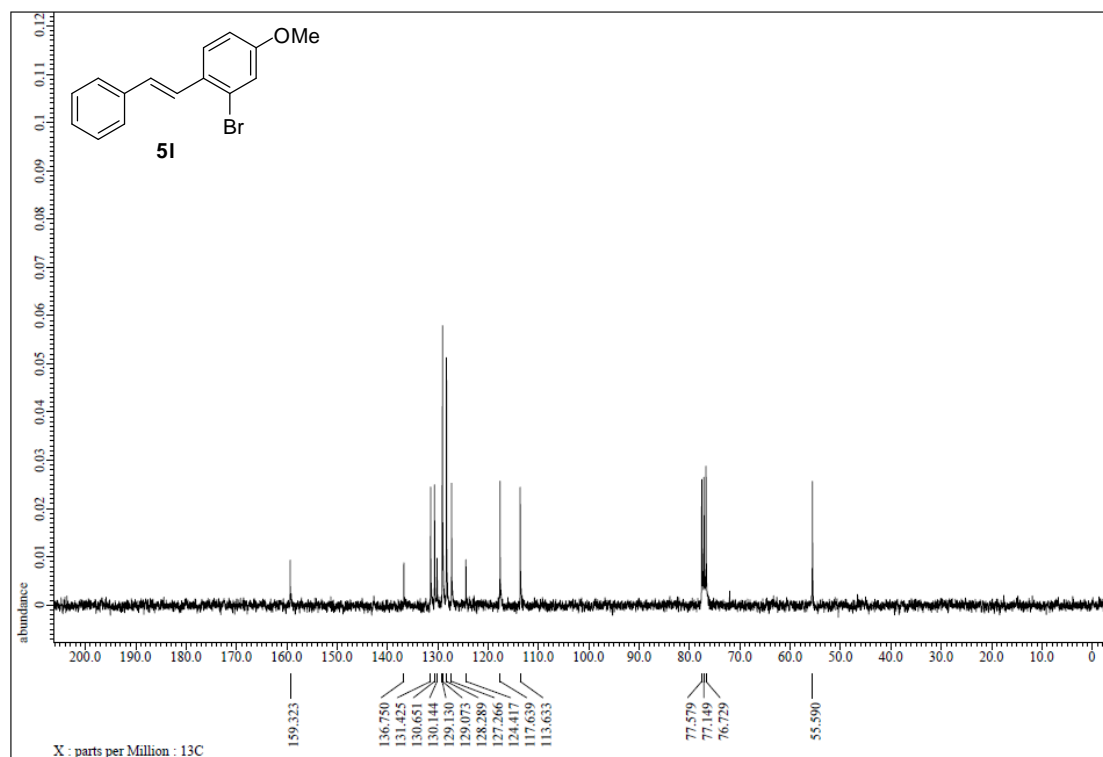
Figure S130. 13 C NMR spectrum of 5I, related to Figure 4.
