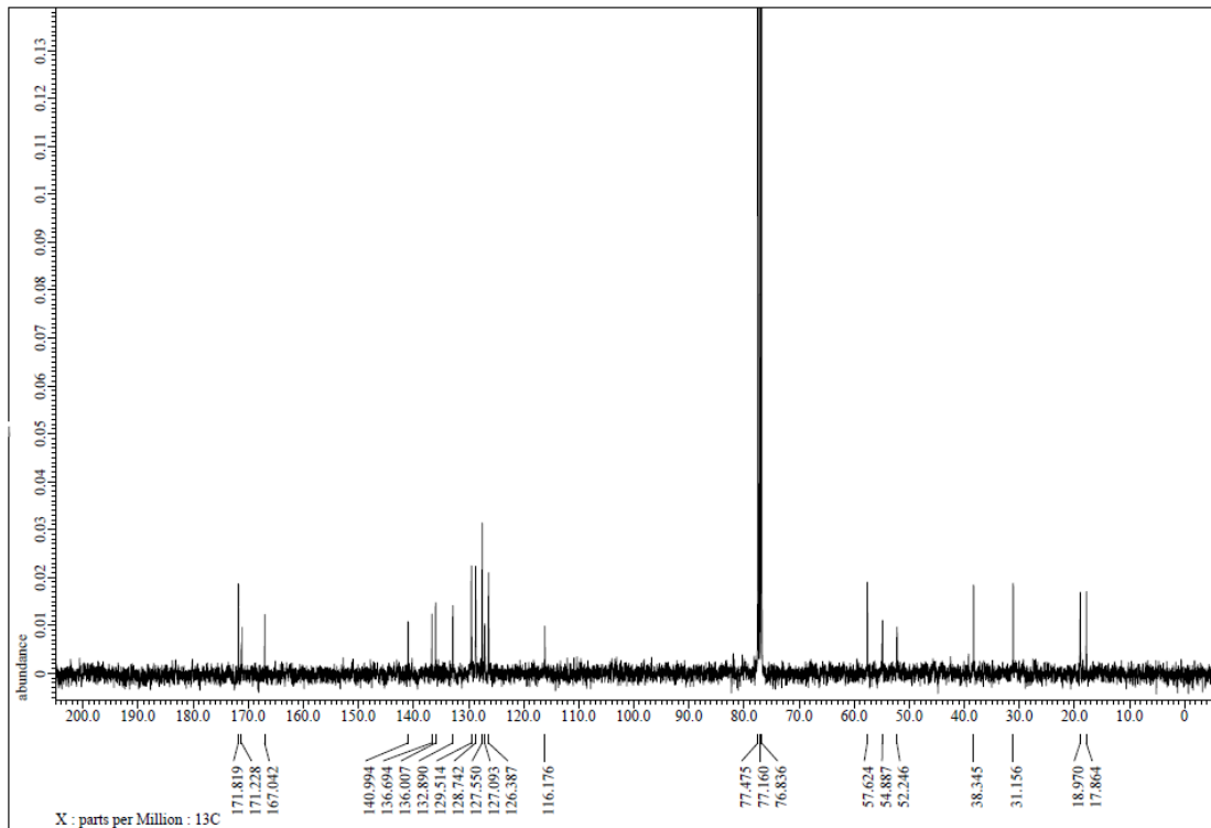
Figure S41. ^{13}\text{C} NMR spectrum of 3s, related to Figure 2.
