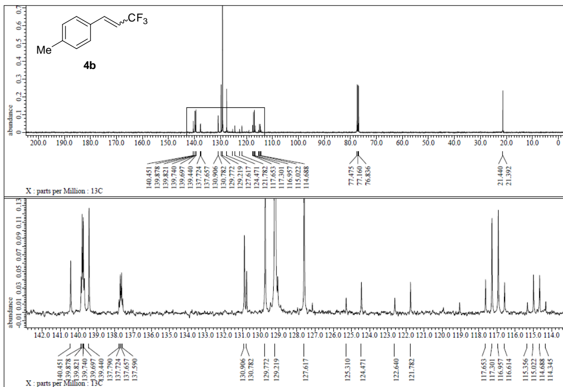
Figure S66. 13 C NMR spectrum of 4b, related to Figure 3.
