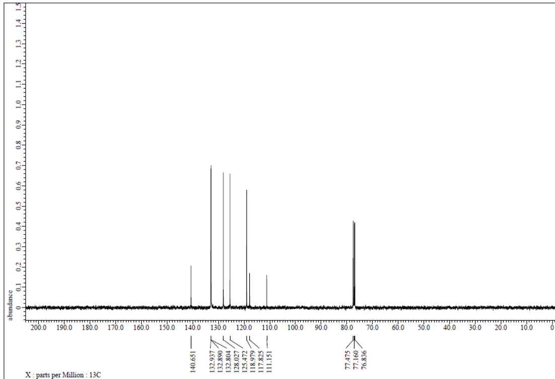
Figure S25. ^{13}\text{C} NMR spectrum of 3k, related to Figure 2.
