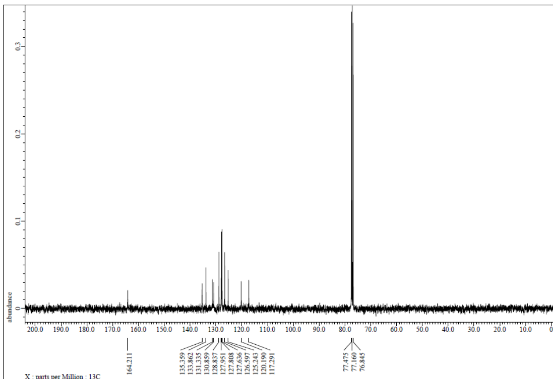
Figure S59. ^{13}\text{C} NMR spectrum of 3ab, related to Figure 2.
