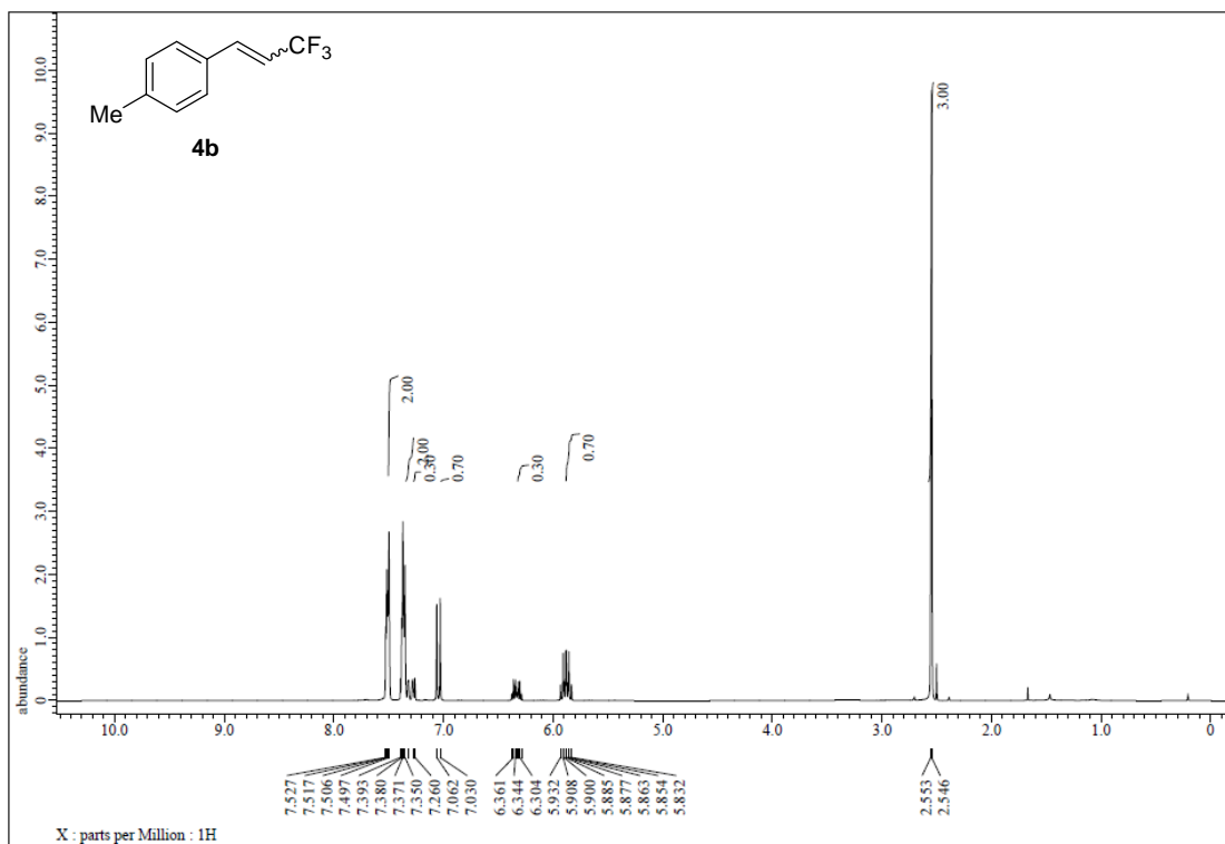
Figure S65. 1 H NMR spectrum of 4b, related to Figure 3.
