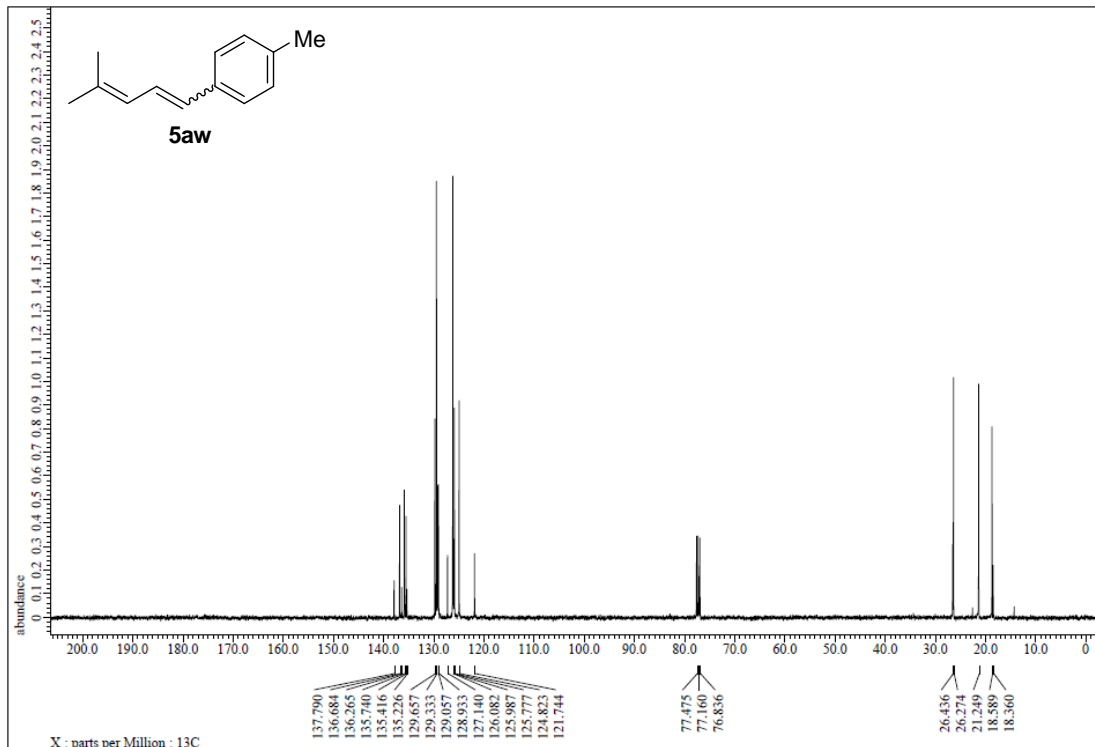
Figure S210. ^{13}\text{C} NMR spectrum of 5aw, related to Figure 5.
