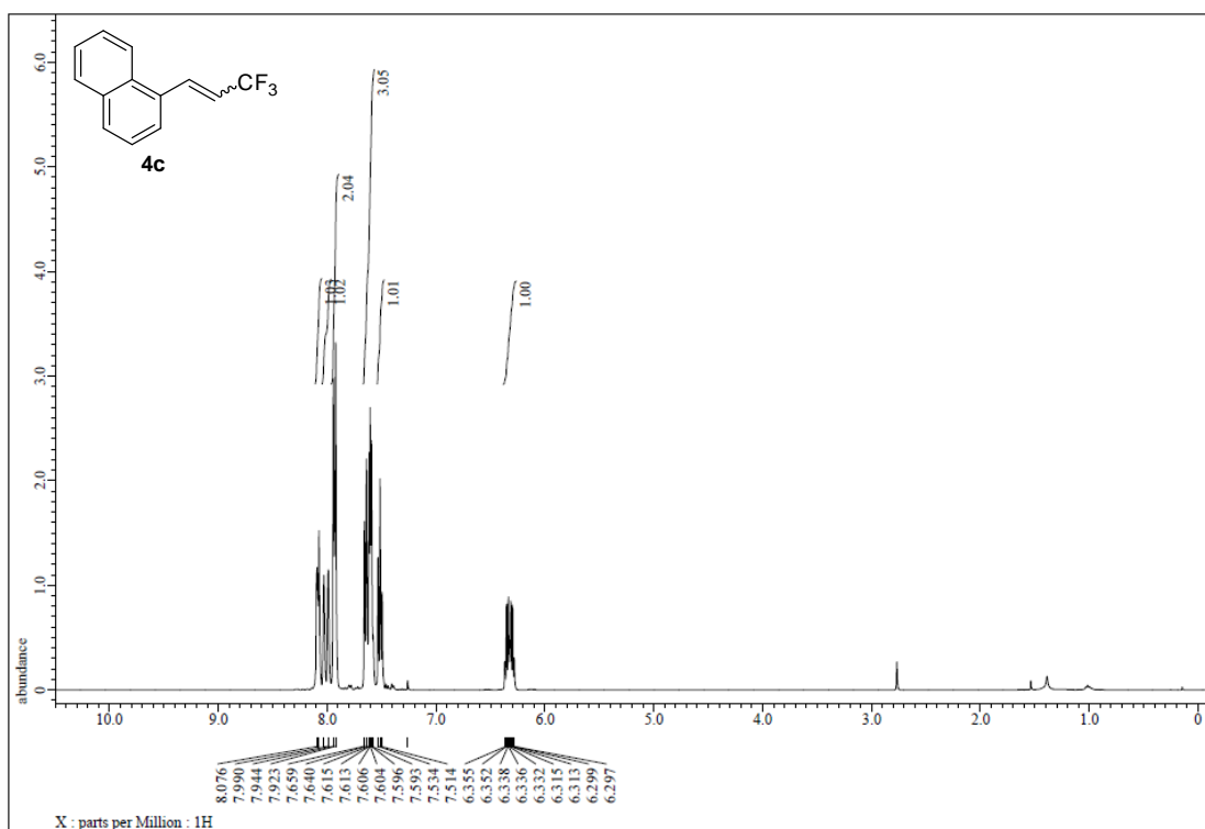
Figure S68. 1 H NMR spectrum of 4c, related to Figure 3.
