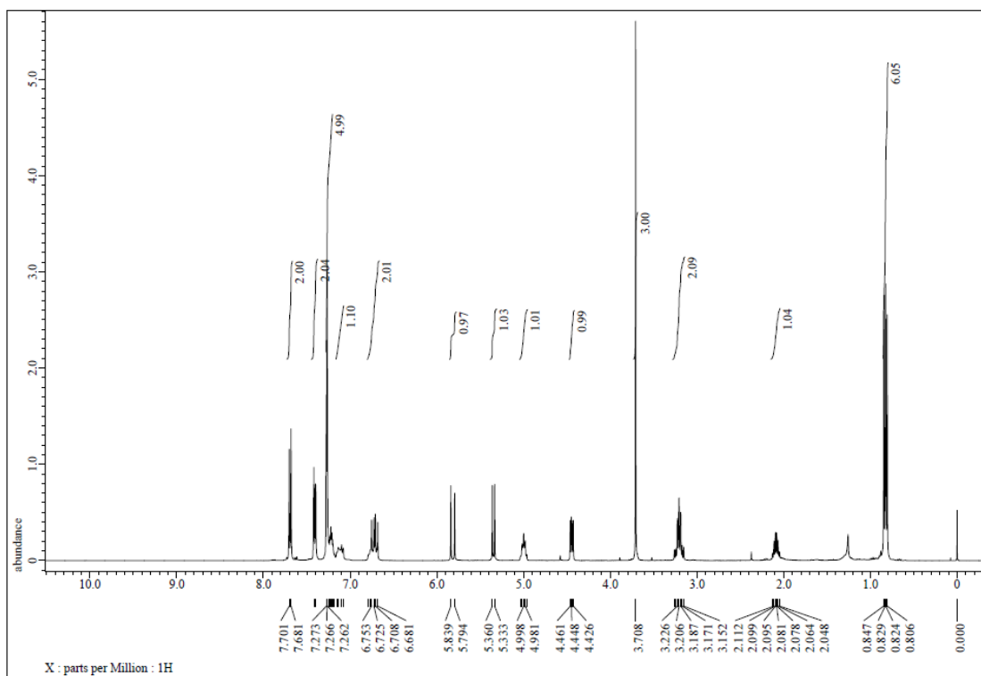
Figure S40. ^1\text{H} NMR spectrum of 3s, related to Figure 2.
