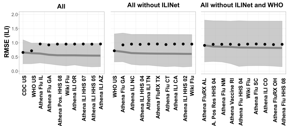
S2 Fig. Performance curves for the first ten selected data sources when all possible data sources are included as candidate predictors ( All ), when ILINet is excluded ( All without ILINet ), and when both ILINet and WHO are excluded ( All without ILINet and WHO ). The system was built through the sequential selection of data sources that minimize average RMSE across 16 out-of-sample forecasts. Selected data are listed in order of inclusion from left to right along the x-axis. Performance is indicated along y-axis in terms of RMSE, with open circles indicating individual performance of selected data sources, and closed circles and shading indicating the mean and range in performance across all 16 out-of-sample forecasts.
