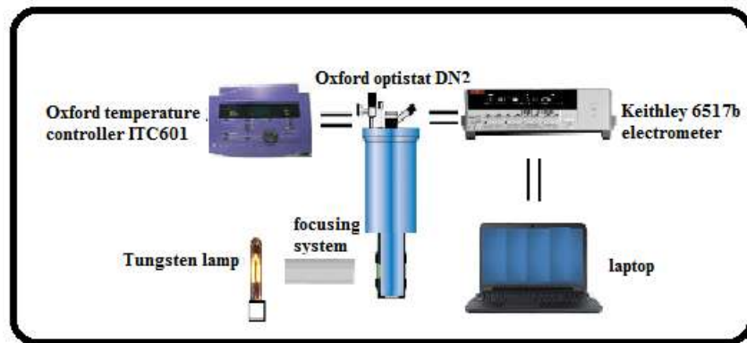
Scheme II: Schematic diagram for photoconductivity measurement
