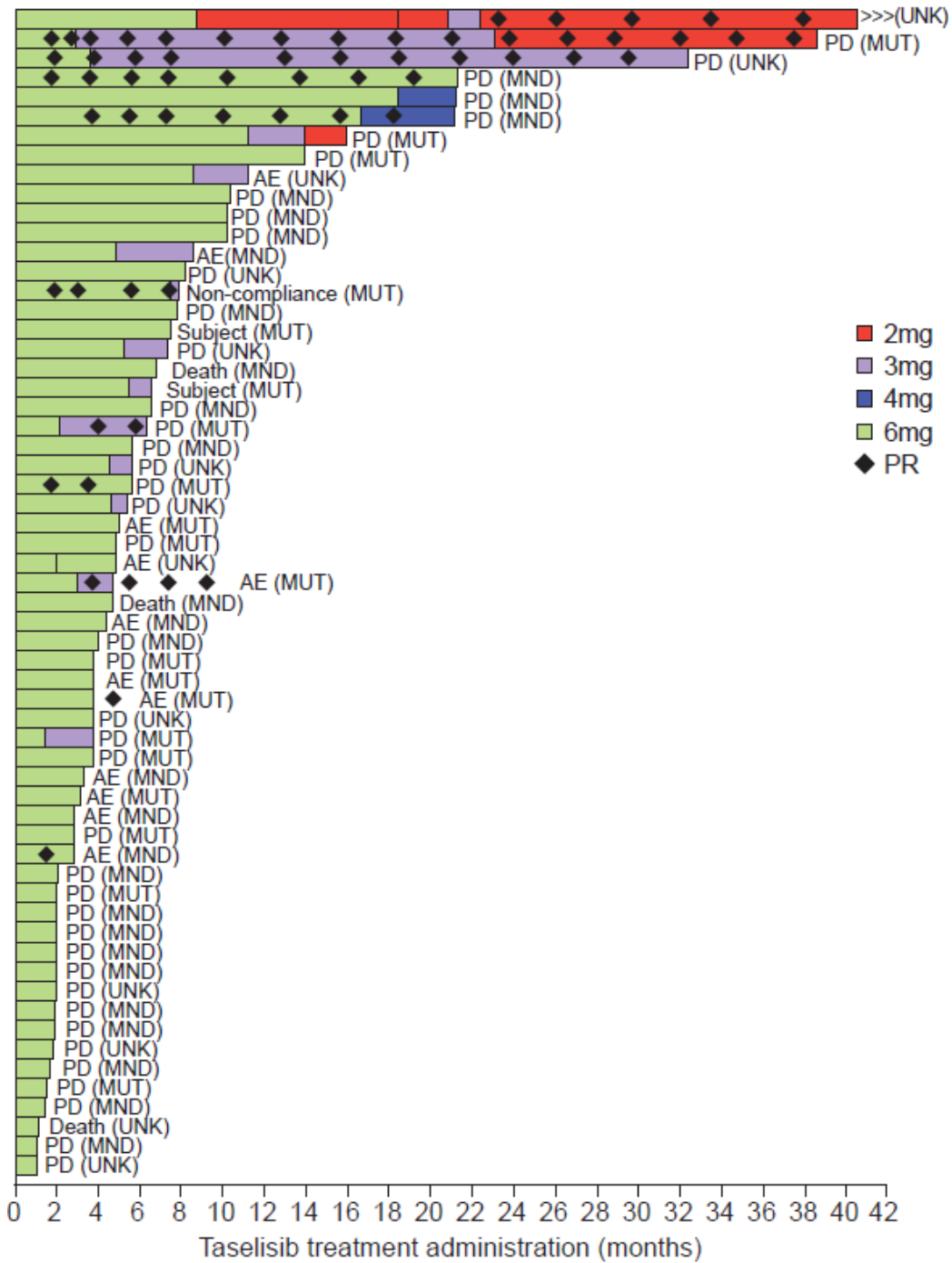
Supplementary Figure S2. Time on treatment by taselesib dose and duration
