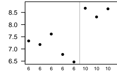
Sh3gl3
