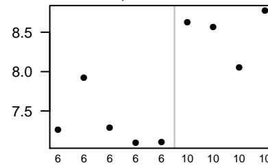
LOC689541
