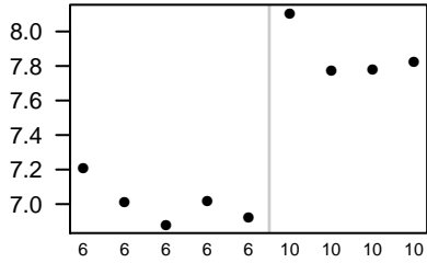
Opalin
