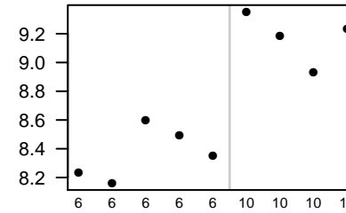
Ceacam10
