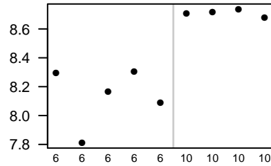
Plp1
