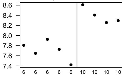
LOC500652
