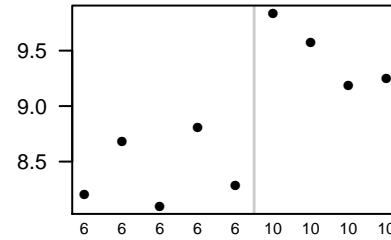
LOC501479
