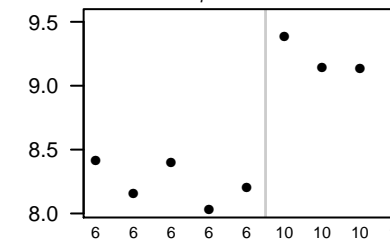
Mbp
