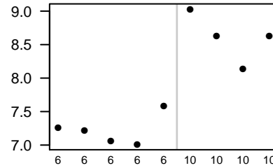
LOC689290
