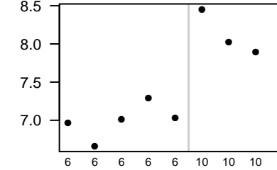
Dhh
