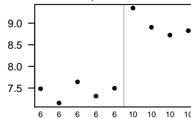
LOC501479
