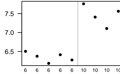
Sema6d_predicted
