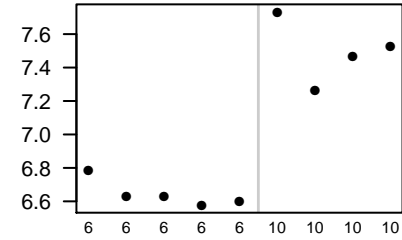
RGD1561090_predicted
