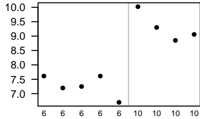
LOC501478
