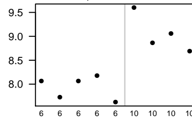
RGD1562608_predicted
