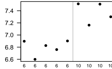
Jam3
