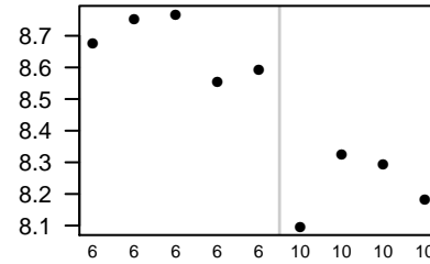
Centd1_predicted
