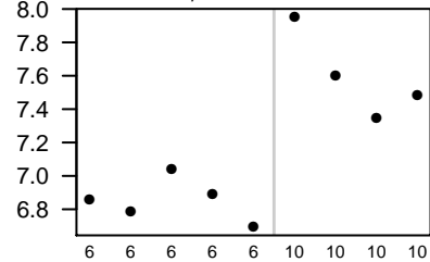
Arfp1
