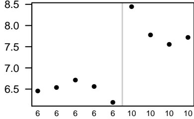
Sema6a_predicted
