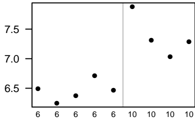
RGD1563633_predicted
