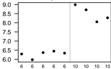
LOC680682
