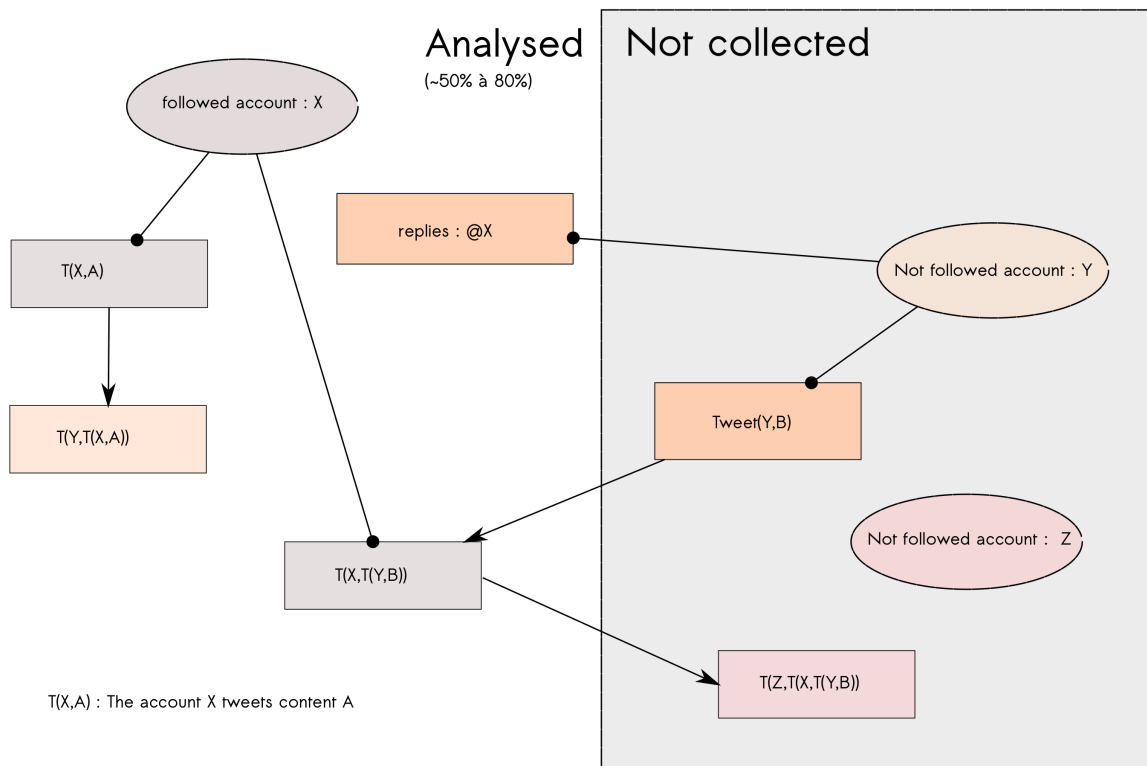
Fig A. Description of the capture protocol centred on political leaders. This is complemented by a keyword-centric capture protocol (Twitter track API).
