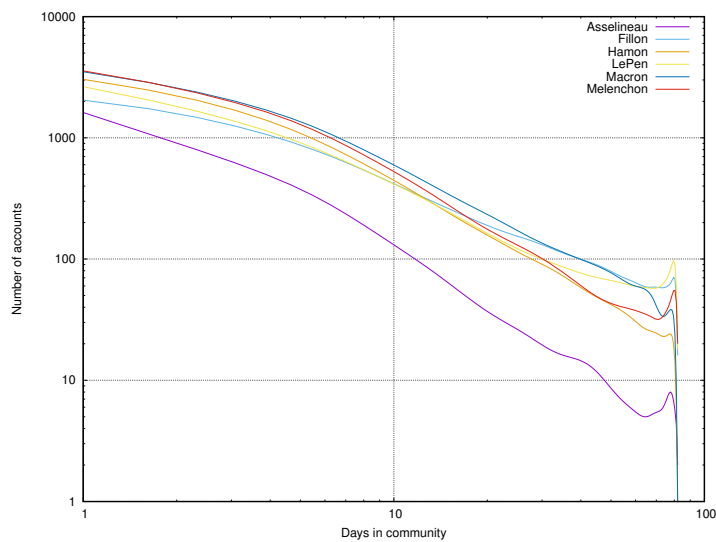
Fig G. Smooth distribution of time spent in a community between July and the 1st round.
