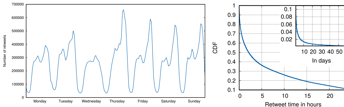
Fig E. Twitter activity patterns. On the left: Number of retweets observed per day and hour between 1 July 2016 and 2 May 2016; on the right: Cumulative distribution of retweet time.
