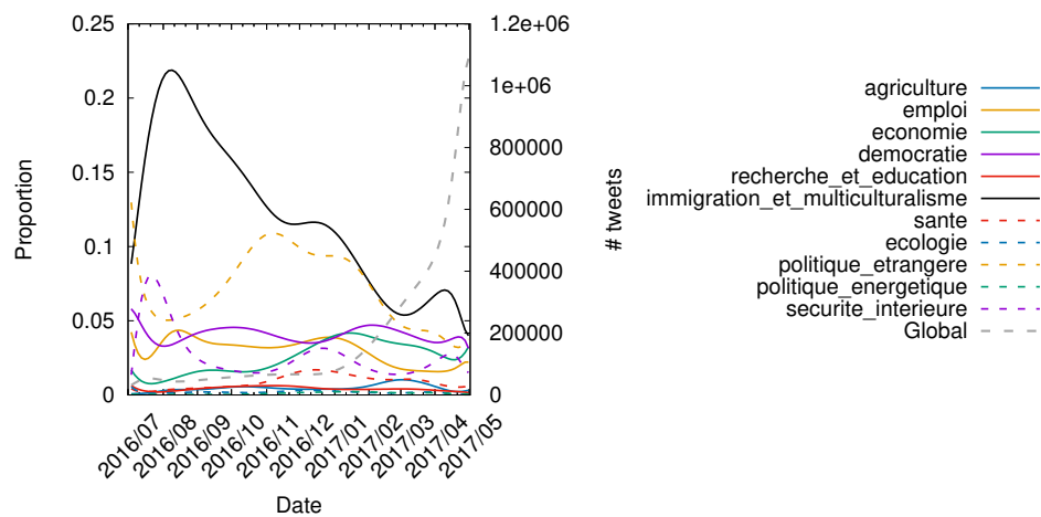
Fig L. Evolution of the topics discussed by the community Marine Le Pen between June 01, 2016 and May 08, 2017.
