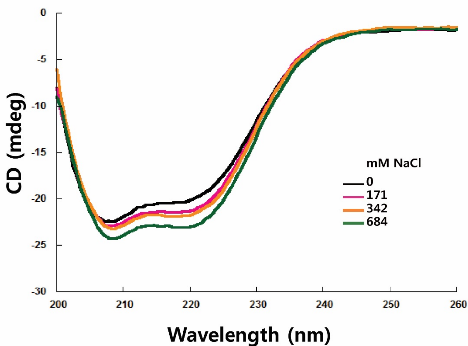
FIG S1 The secondary structure of Im7 L53A I54A was monitored by circular dichroism spectroscopy at 10°C. 20 \mu M of proteins in 20 mM sodium phosphate buffer at pH 7.2 containing NaCl concentrations ranging from 0 to 684 mM were used.
