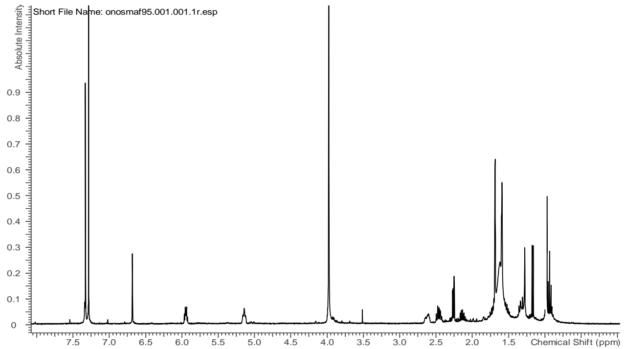
H-NMR of compound 11
