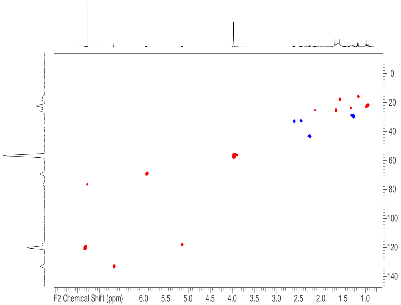
HSQC of compound 11
