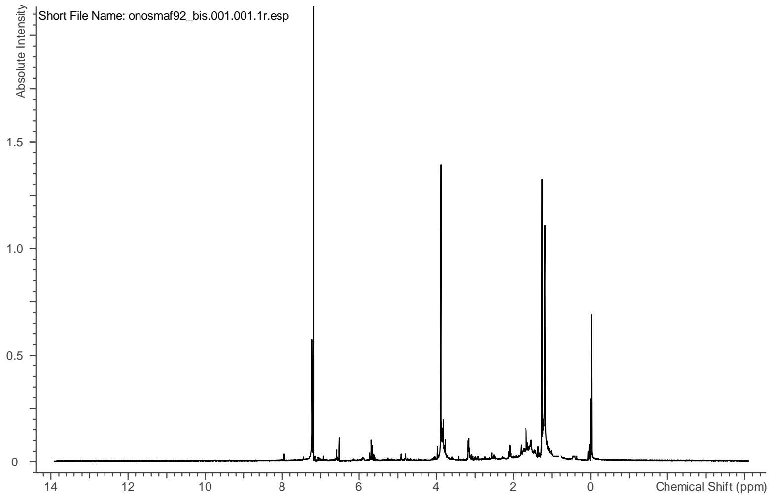
H-NMR of compound 8
