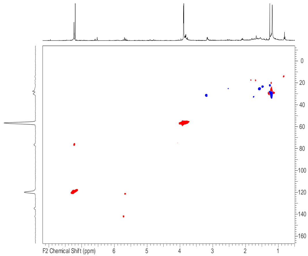
HSQC of compound 8
