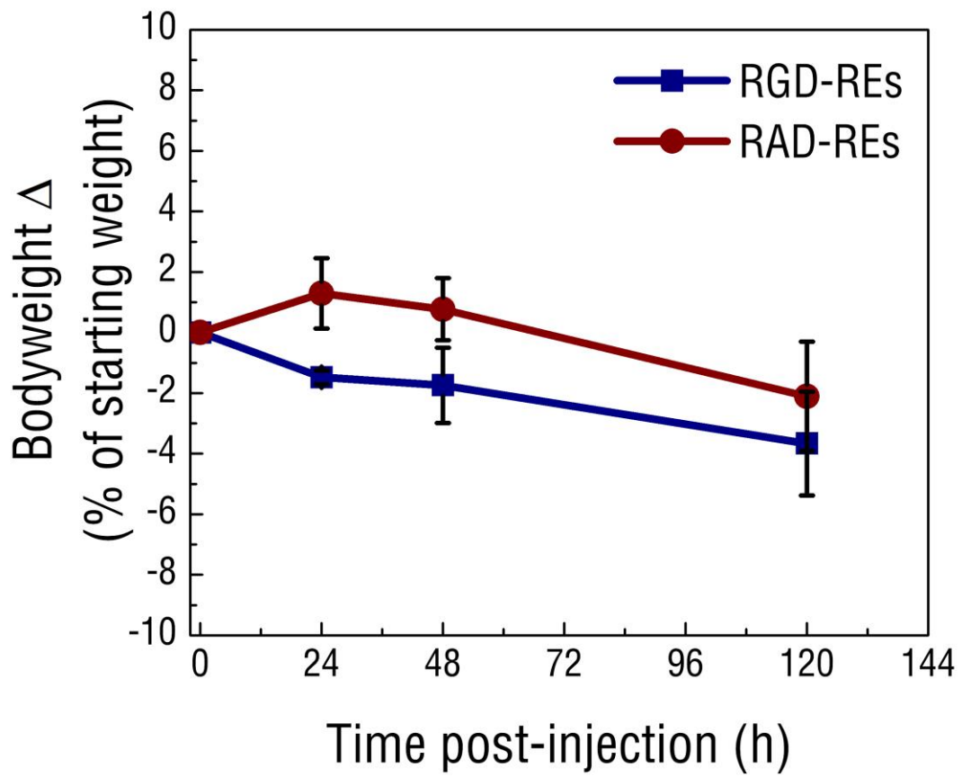
Supplemental Figure S4 – Changes in the bodyweight of mice exposed systemically with functionalized REs.
