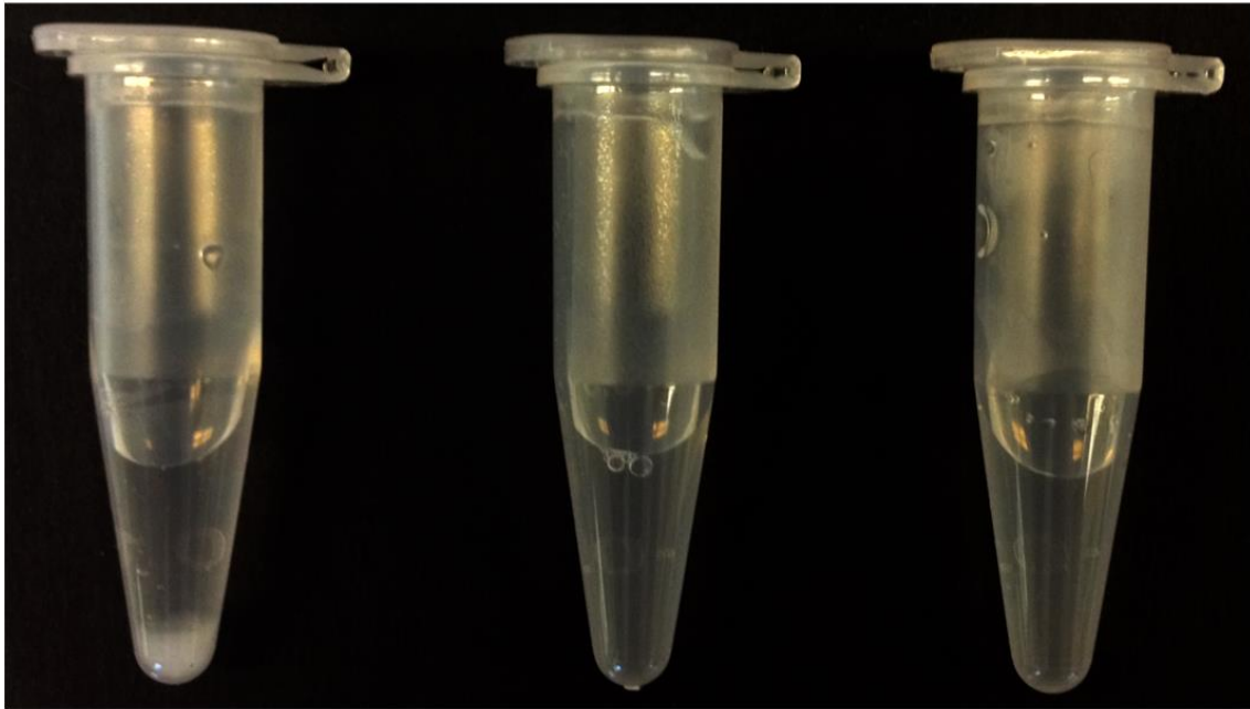
Supplemental Figure S1 - Image of various formulations of REs in solution shows that in contrast to the as-synthesized REs, both PEGylated and functionalized REs are readily dispersed in aqueous buffer.
