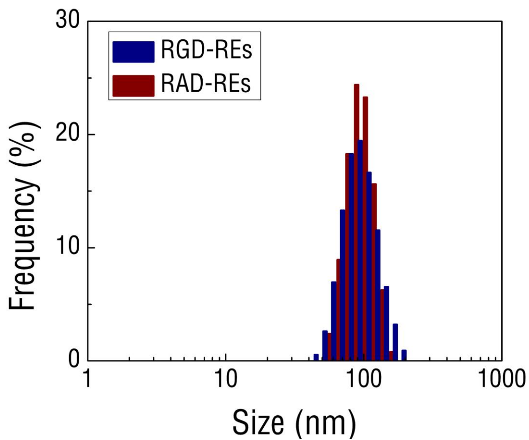
Supplemental Figure S3 – Size distribution of functionalized REs in PBS shows similar, narrow size Distribution.
