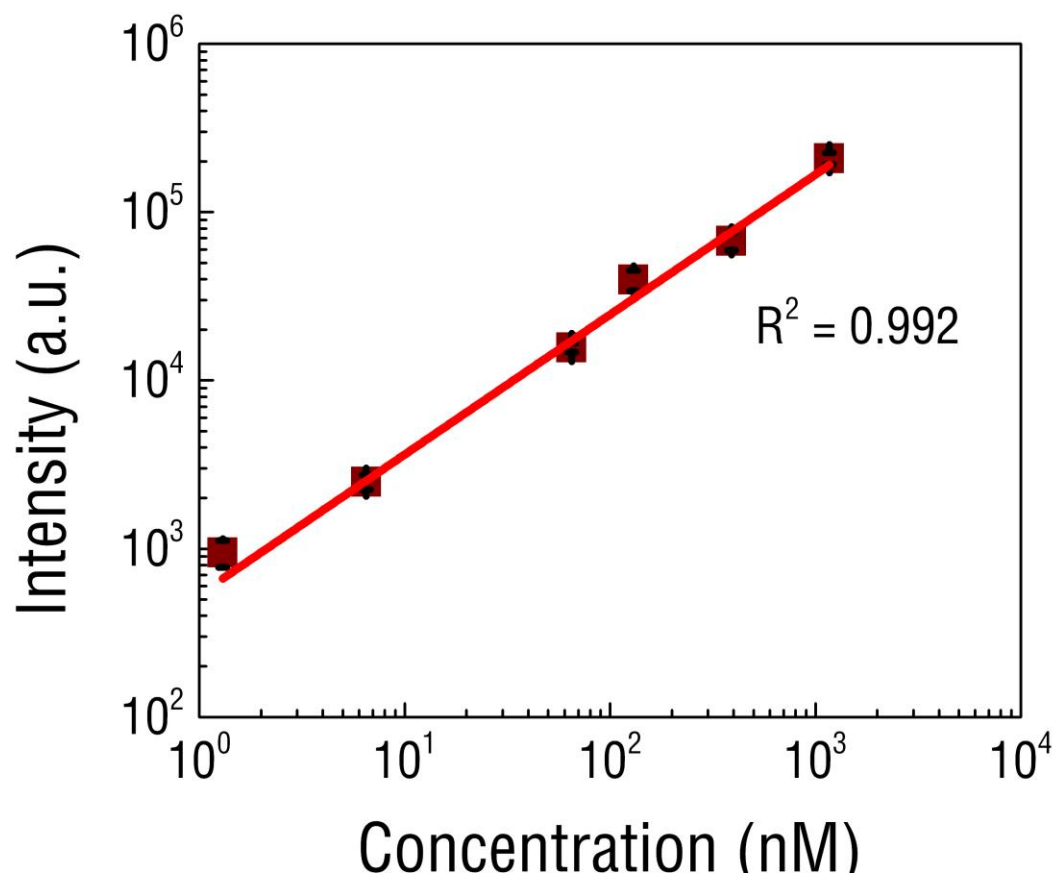
Supplemental Figure S2 – Calibration curve of the SWIR imaging system through serial dilution of REs reveals a strongly linear relationship between SWIR signal intensity and RE concentration.
