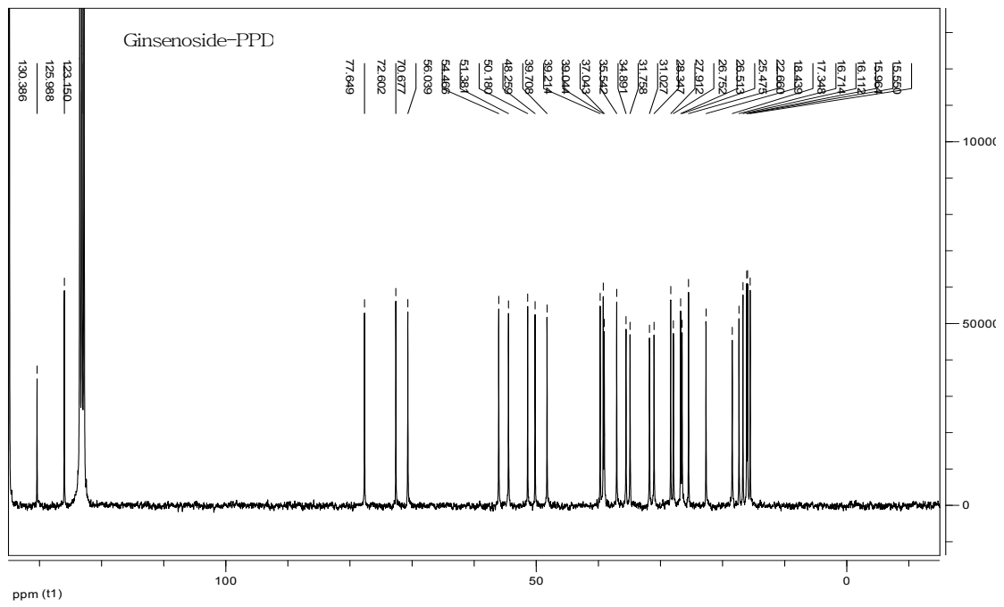
Figure 3. ^{13}\text{C} NMR of PPD.
