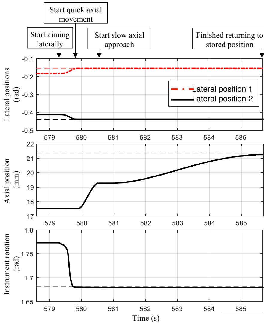
Figure 4. Instrument movement during ‘return to stored position’. Dashed lines denote previously stored positions.
