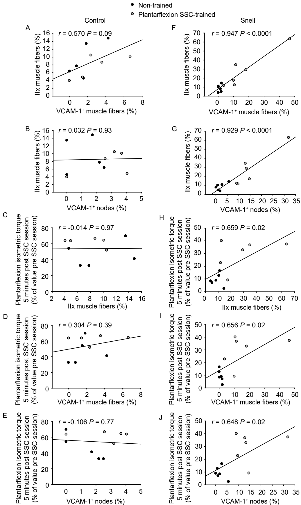
Fig. S4. A robust and coordinated remodeling response in VCAM-1 and type IIx fiber distribution unique to SSC-trained Snell dwarf mice was correlated with improved recovery from fatigue. Correlations between VCAM-1 + staining, type IIx fibers, and post-SSC isometric torque (a measure of fatigue recovery) were determined for (A-E) control mice and (F-J) Snell dwarf mice. Correlation coefficients and P values were determined by Pearson product correlation analysis. Sample sizes were N = 5 to 6 per group.
