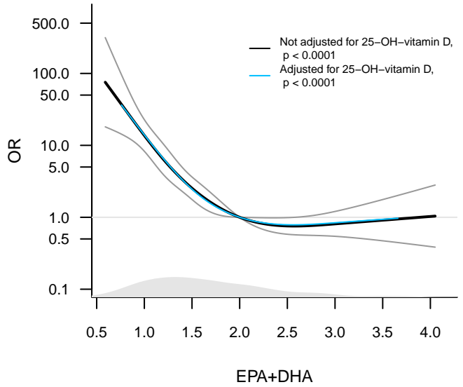
2nd sample, adjusted for covariates
