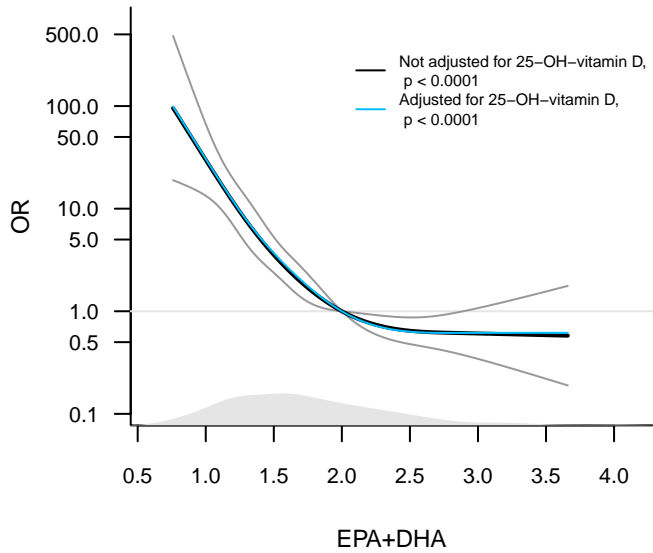
Mean of 1st and 2nd sample, adjusted for covariates
