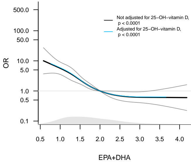
1st sample, adjusted for covariates
