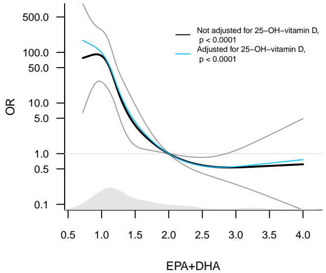
Concordent quintiles, adjusted for covariates
