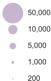
Contig lengths
