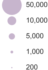
Contig lengths
