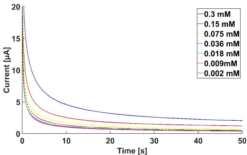
Figure S1. Amperometric measurements using the optimized potential of 0.78 V on different concentrations of glyphosate using a gold working electrode.
