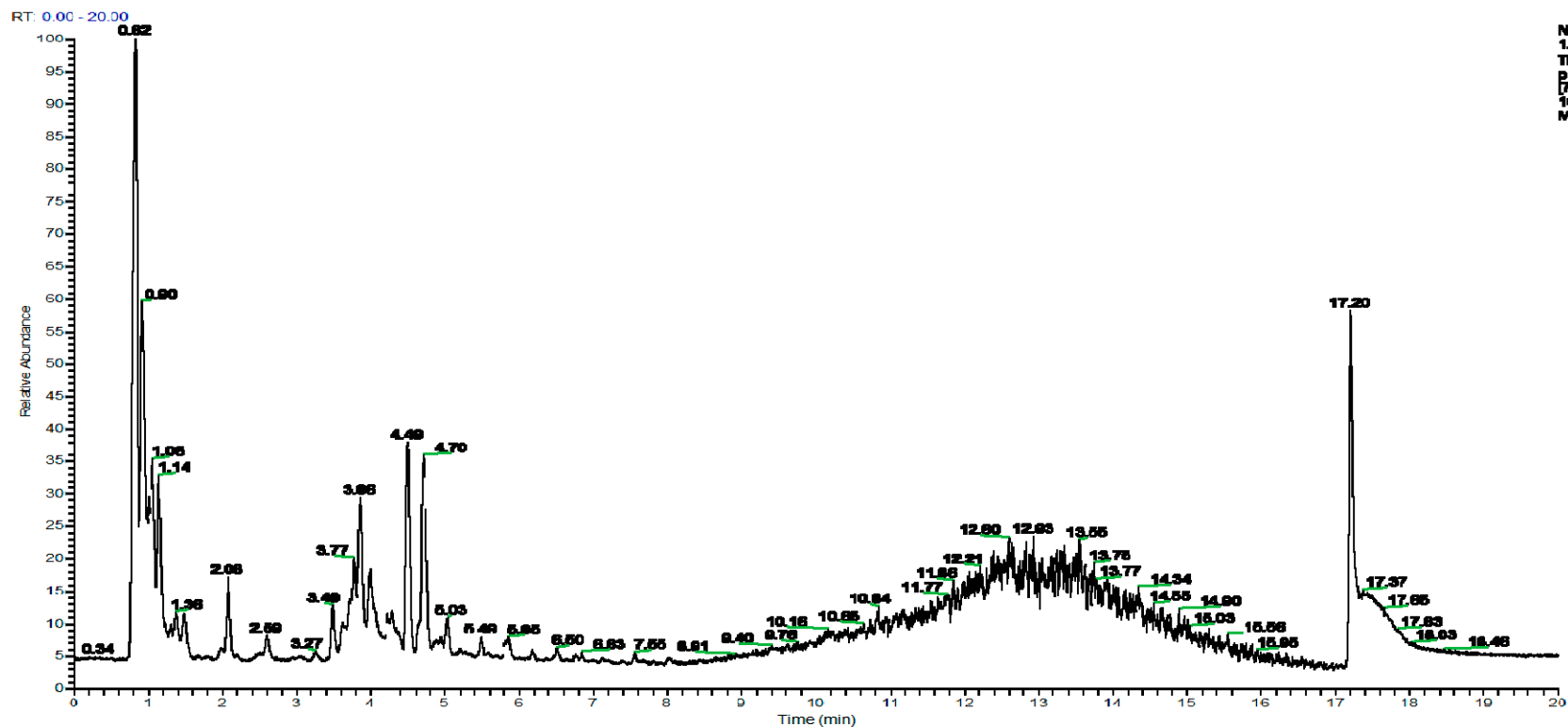
Supplementary Figure 1-Total ion chromatogram-summing up intensities of all mass spectral peaks of SLT by UPLC-Q-Orbitrap; TIC(+POS)-Positive ion mode.
