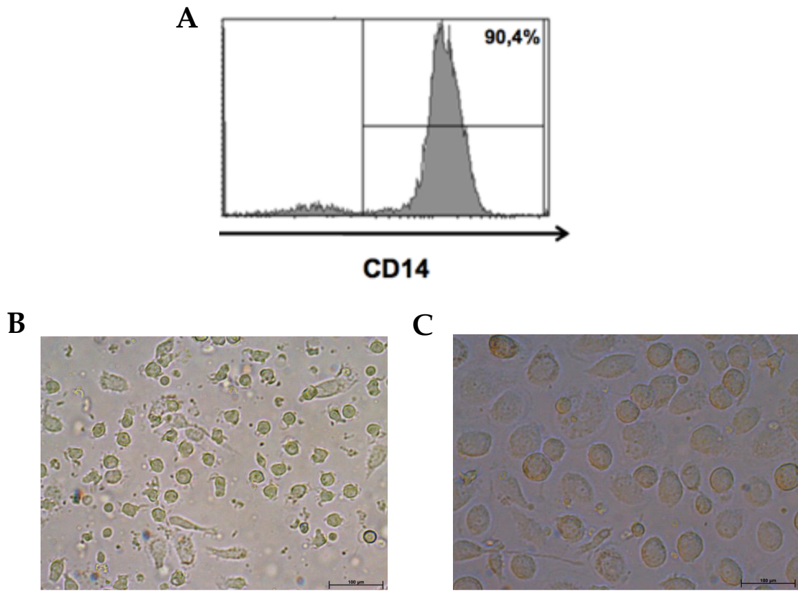
Figure S1. Morphological development of human monocyte-derived macrophages (MDMs). Freshly isolated monocytes obtained from PBMCs by positive selection were stained with an anti-CD14 antibody (A). Cell morphology of monocytes cultured for 1 day (B) and after 7 days of differentiation (C) is shown. Bar correspond to 100 μm.
