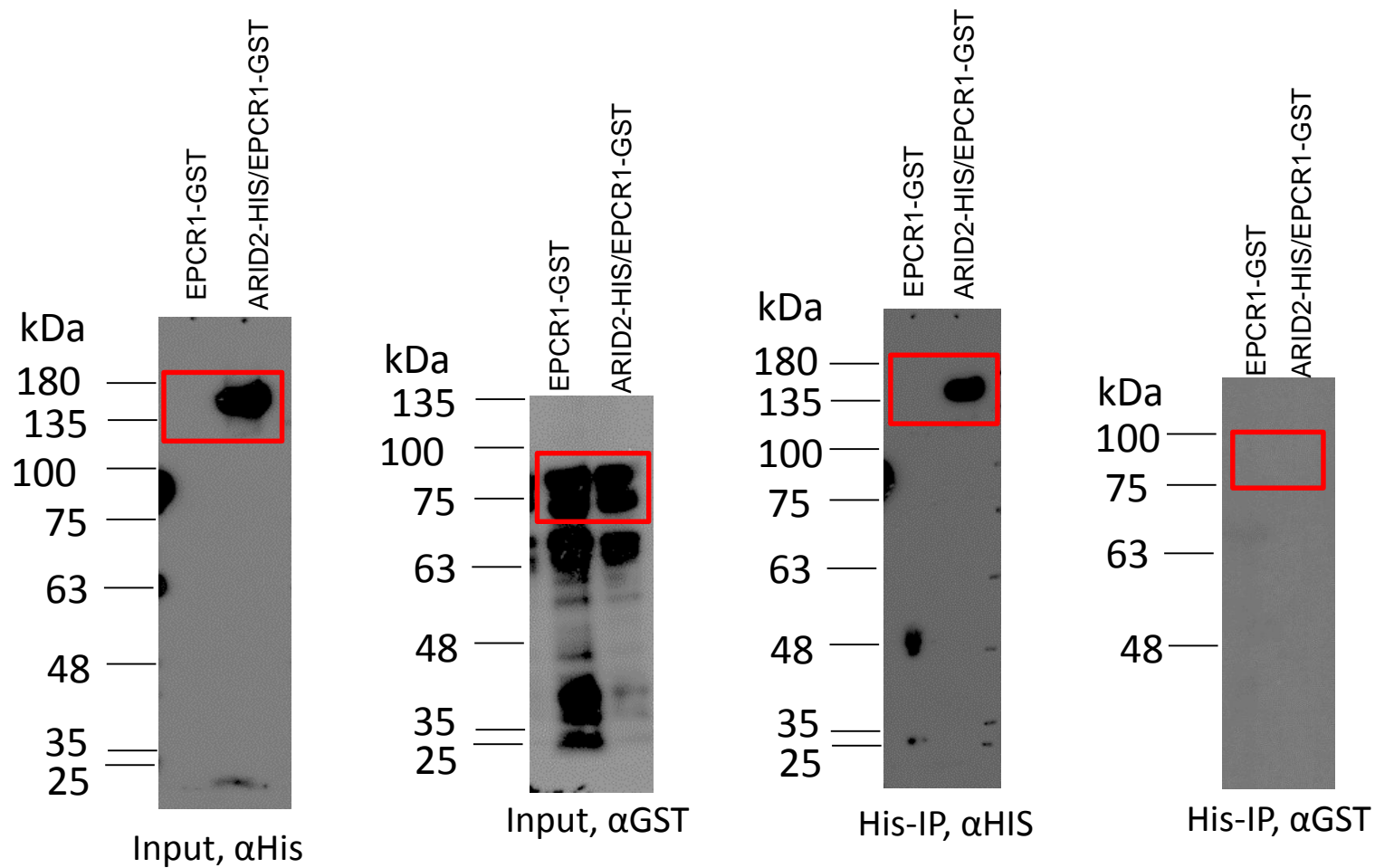
Fig 2F EPCR1-GST/ARID2-HIS
