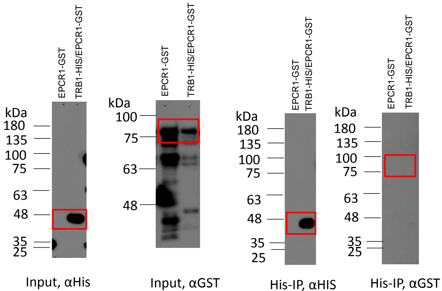
Fig 2F EPCR1-GST/TRB1-HIS
