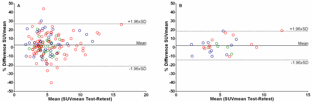
Supplemental Figure 1. Bland–Altman plots showing repeatability of SUV_{mean} on lesion (A) and patient (B) level. (Blue: Center 1; Red: Center 2; Green: Center 3)
