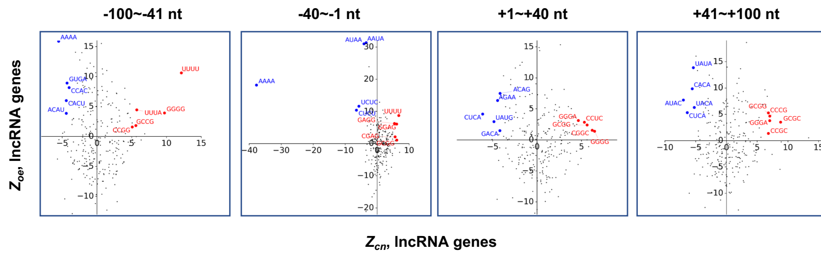
Figure S11. Comparison of sequence motifs between conserved and nonconserved PASs in four regions around the PAS. Data are shown as in Figure 7F, except that all four flanking regions (-100 to -41 nt, -40 to -1 nt, +1 to +40 nt, and +41 to +100 nt) of mRNA PASs (A) and lncRNA PASs (B) are shown. See Figure 7F legend for definitions of Z oe and Z cn .
