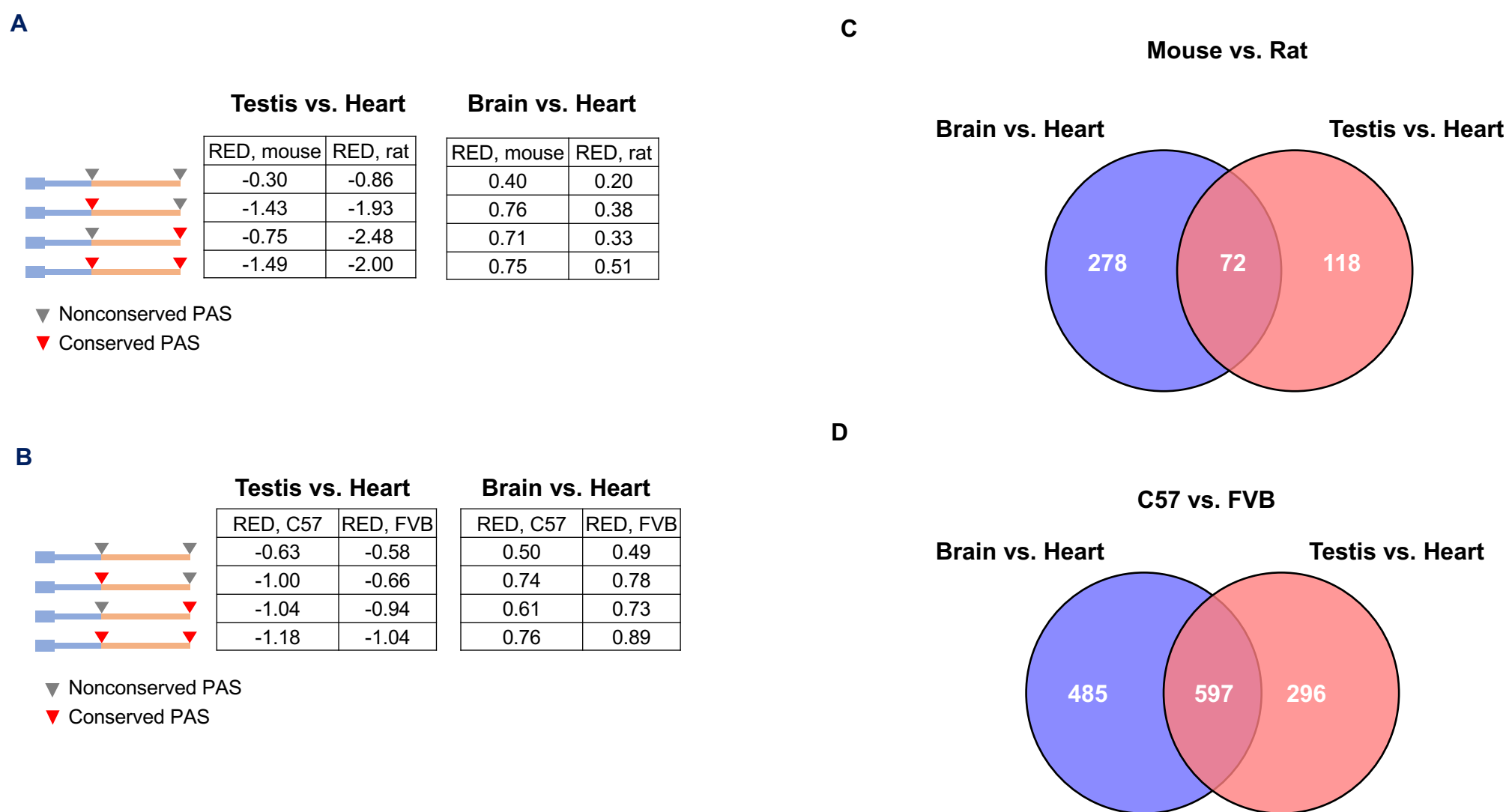
Figure S9. Global APA trends between tissues. (A) RED (testis vs. heart or brain vs. heart) of four types of genes in mouse and rat. The definition of gene type is the same as in Figure 5E. (B) RED (testis vs. heart or brain vs. heart) of four types of genes in two mouse strains (C57 vs. FVB). The definition of gene type is the same as in Figure 5G. (C) Venn diagram of genes with poorly correlated APA events between mouse and rat as defined in Figure 6A. (D) Venn diagram of genes with poorly correlated APA events between mouse strains as defined in Figure 6D.
