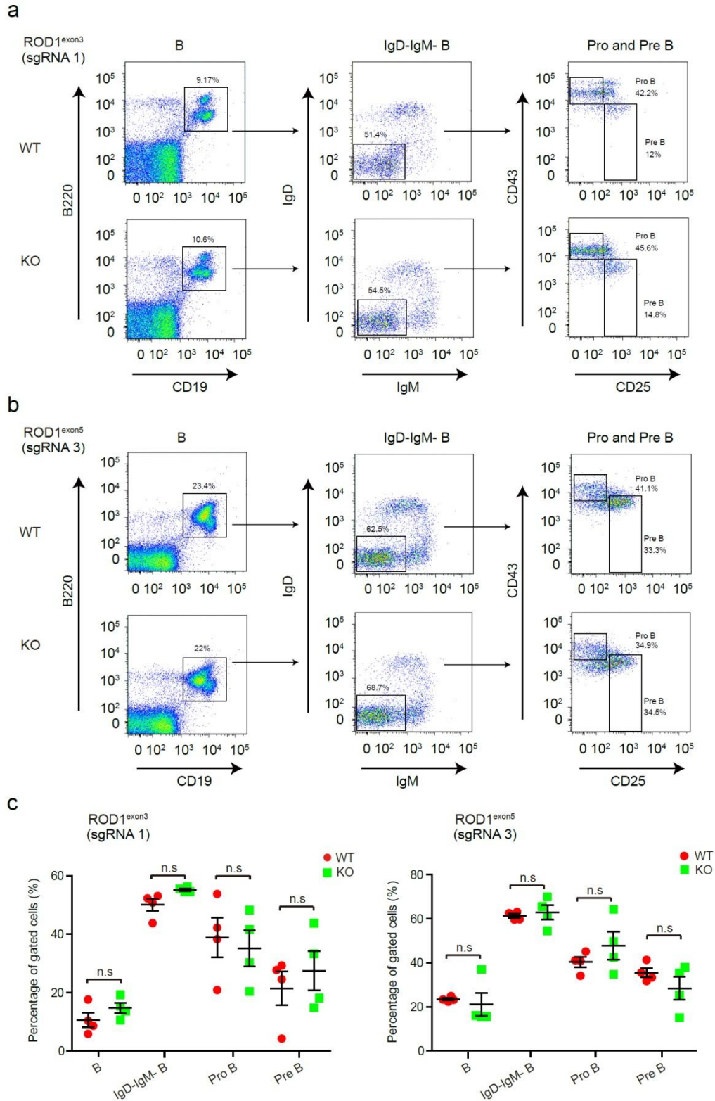
Supplementary Figure 10. ROD1 ablation has no influence on B cell differentiation in the bone marrow of muMT chimeric mice. (a, b) Flow cytometric analysis of repopulating bone marrow B cells in muMT and WT or ROD1 -/- chimeric mice after 6
