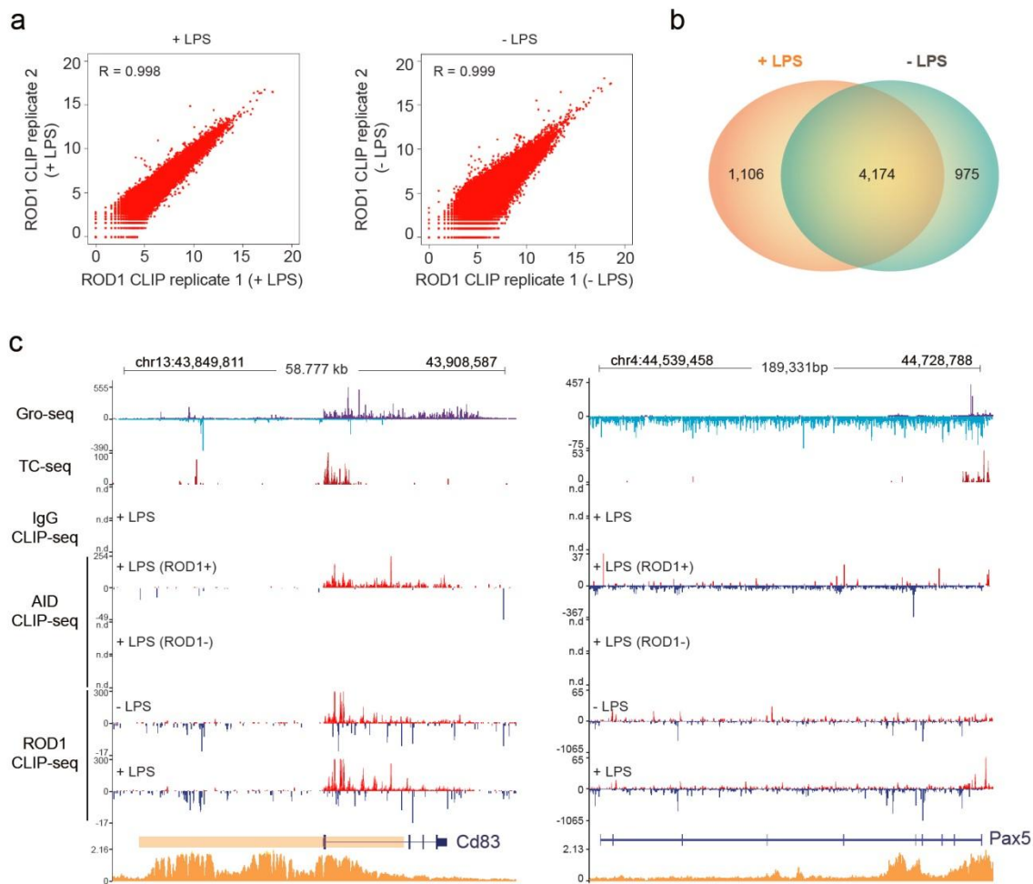
Supplementary Figure 13. ROD1 binding profiles are similar before and after LPS stimulation. (a) Pearson's correlation analysis of ROD1 CLIP-seq replicates. (b) Venn diagram of genes with ROD1 CLIP-seq peaks before and after LPS treatment. (c) Snapshot of the Gro-seq, TC-seq and CLIP-seq profiles in the vicinity of Pax5 and Cd83 . ROD1 and AID CLIP-seq signals are shown as red and blue for reads located on the Watson and Crick strands, respectively. Bottom: the H3K27Ac signal is shown in orange. The reported super-enhancer is marked with an orange box.
