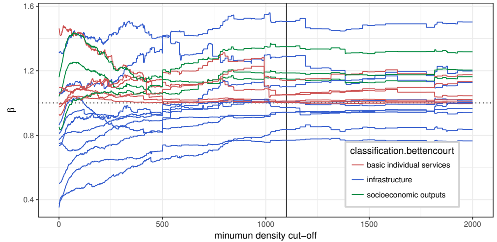
S1 Fig Scaling exponent \beta as a function of minimum density cut-off for all the variables. Each line represents the scaling exponent (y-axis) from OLS regressions of the log-transformed data of each variable as a function of the minimum density cut-off (x-axis).
