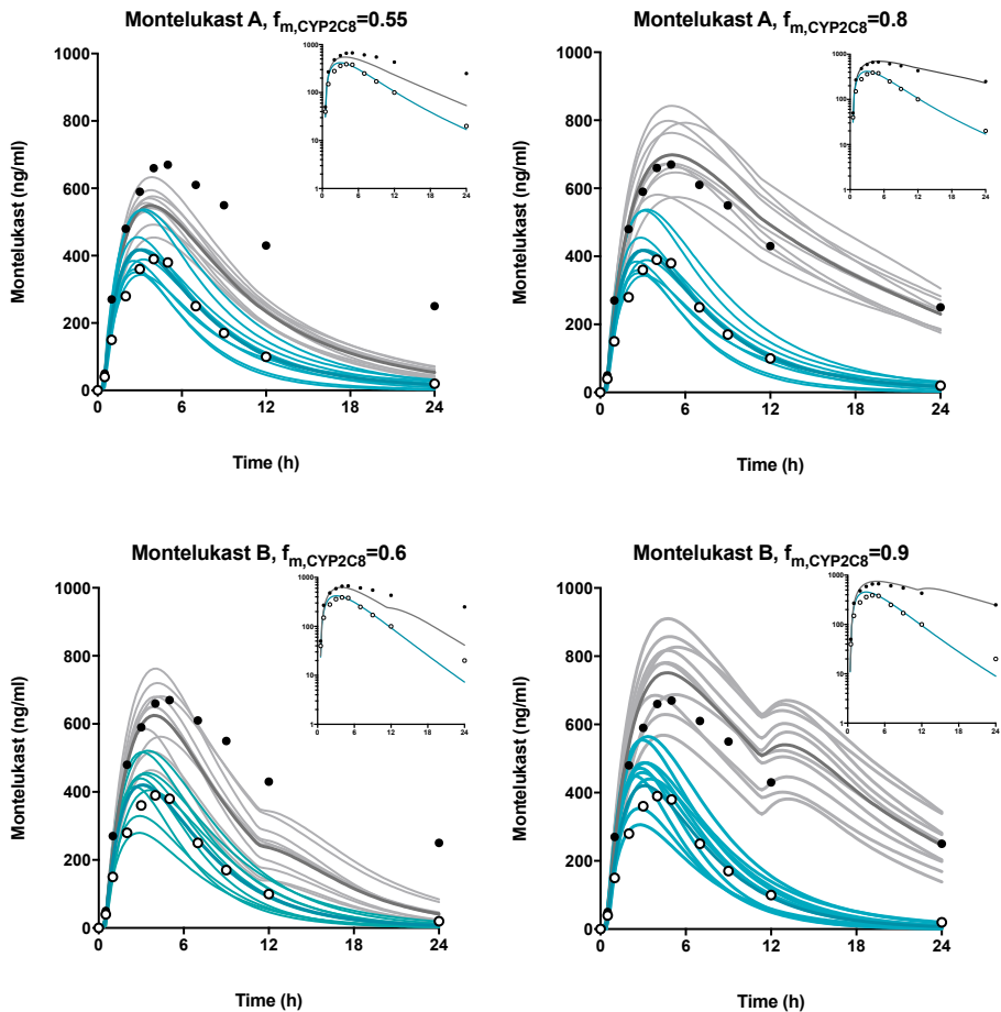
Figure S4. PBPK simulations demonstrating the effect of gemfibrozil on the plasma concentrations of montelukast A (perfusion-limited model) and montelukast B (permeability-limited model with OATP1B1 transport, when montelukast f_{m,CYP2C8} varies between 0.55 and 0.9). Individual trials are shown as thin lines, and their means as thick lines. Blue lines represent the placebo phase and grey lines the gemfibrozil phase.
