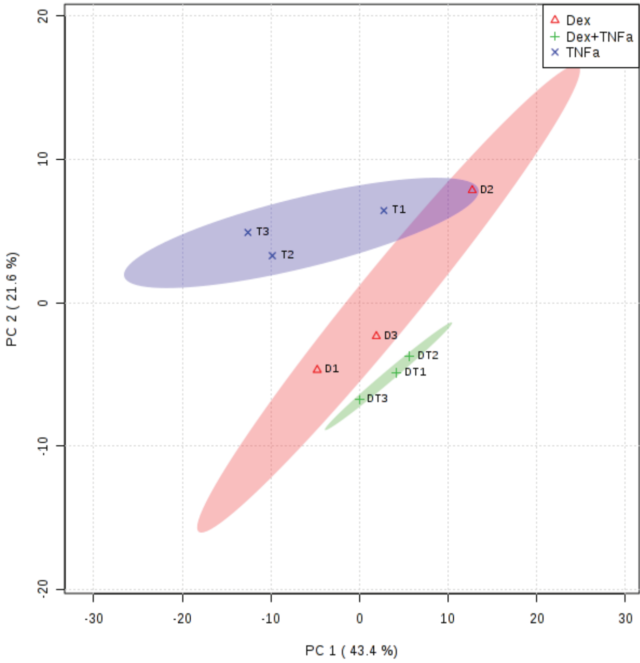
Scores Plot
