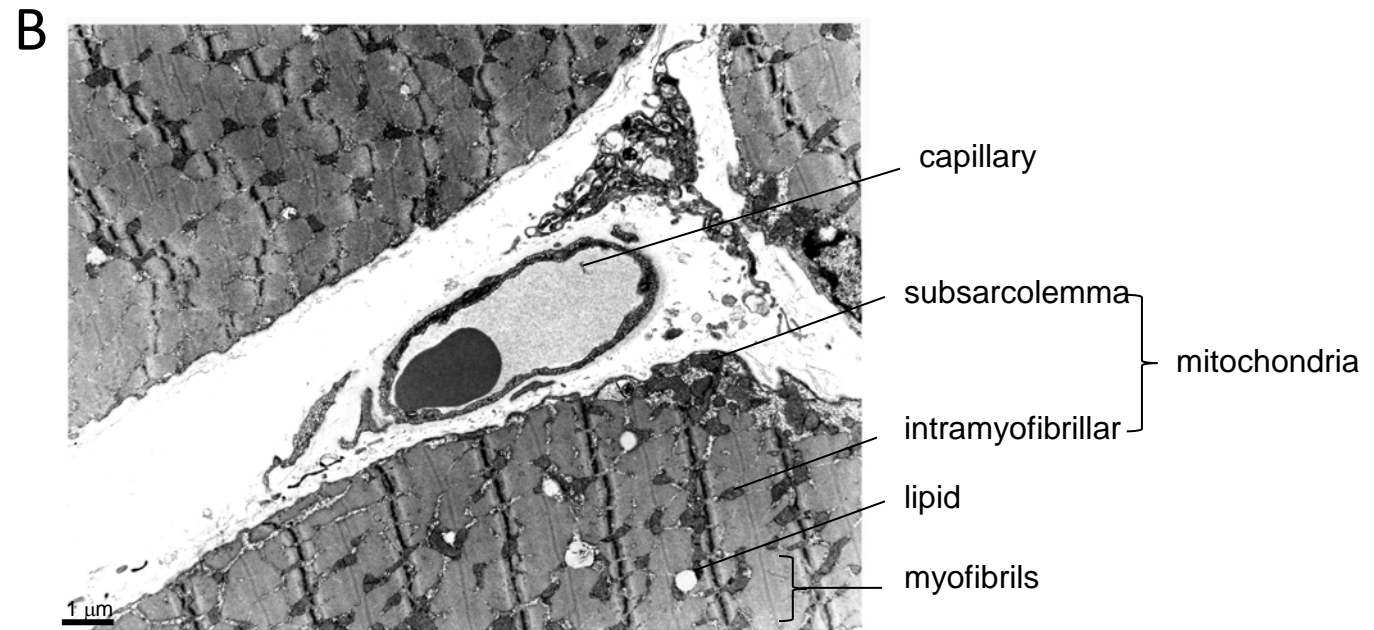
Supplementary Figure S1: Illustration of measured cellular parameters. A,B) Photographic record of alkali stable myofibrillar ATPase in cross-sectioned muscle fibers (A) and electron micrograph (B) from a vastus lateralis biopsy of a contralateral control. Examples of the quantified cellular and ultrastructural parameters are indicated.
