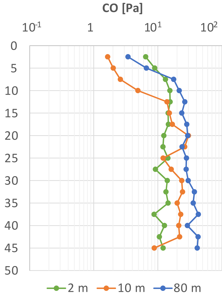
Figure S1. Carbon monoxide pools measured in sediment cores taken in Lake Constance at three different water depths (2 m, 10 m, 80 m).
