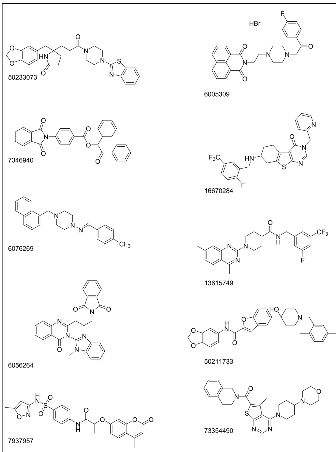
Supplementary Figure 1: The different molecules that potentially bind open state tTG. Our virtual screen identified 24 molecules that could preferentially dock onto open state tTG. The structure and corresponding ChemBridge catalog number of each molecule is shown. Compounds in the manuscript are designated TTGM #, where # is the final four digits of each compound's catalog code.
